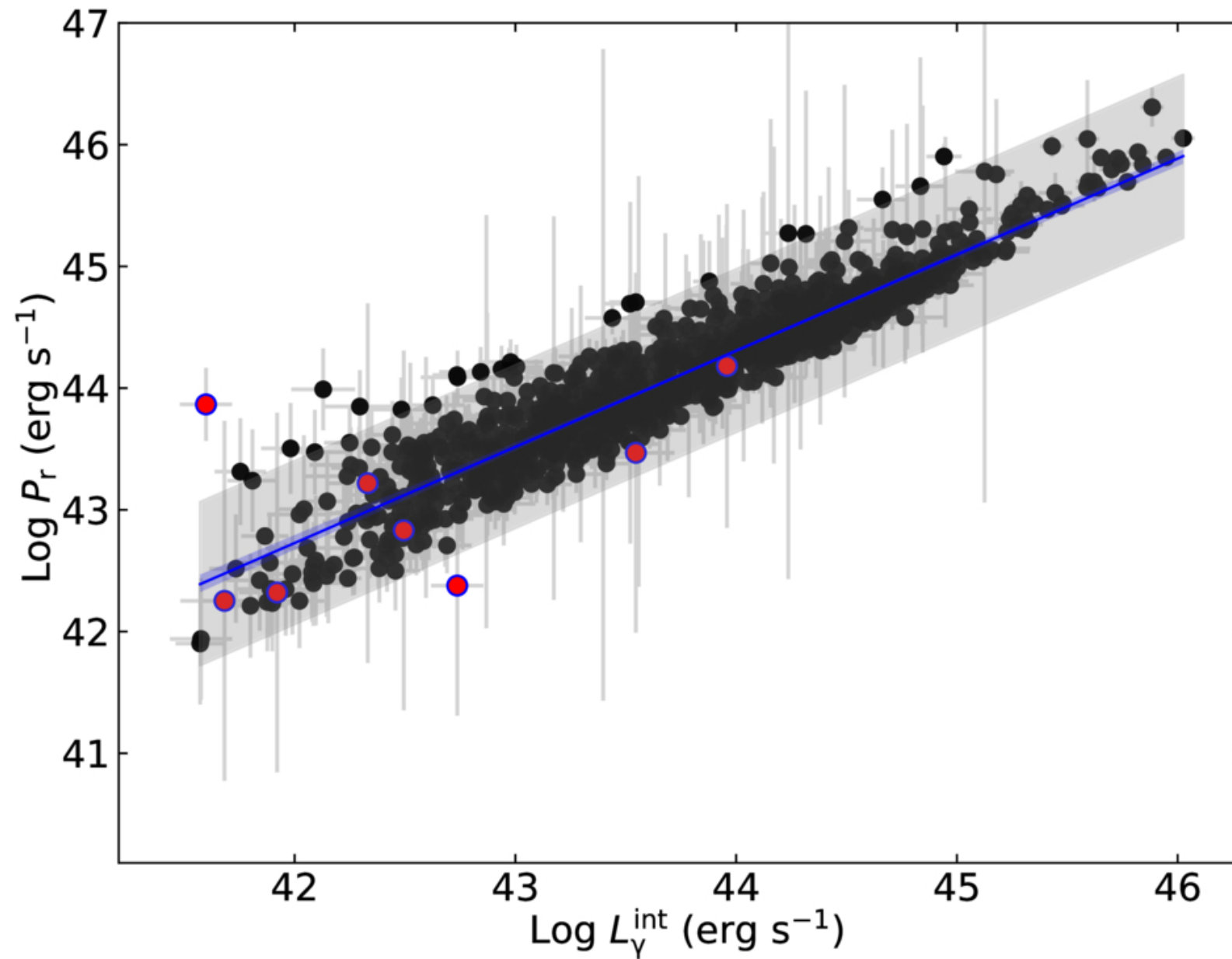
Figure 2. from Dingrong Xiong et al 2026 Astrophys. J. 1009 doi:10.3847/1538-4357/ae9a92 https://dx.doi.org/10.3847/1538-4357/ae9a92 © 2026. The Author(s). Published by the American Astronomical Society.
