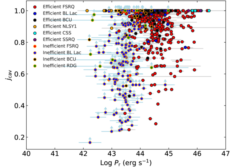
(b) Black hole spin versus jet radiative power assuming that P_{\text{kin}} = P_{\text{cav}}
