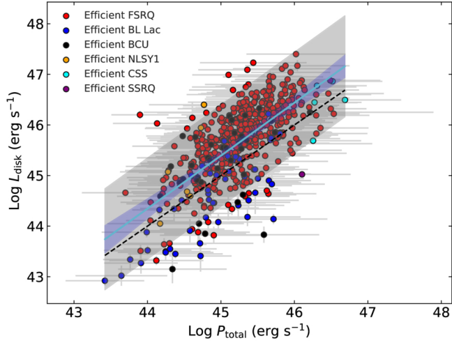
(a) Total jet power versus accretion disk luminosity in radiatively efficient AGNs
