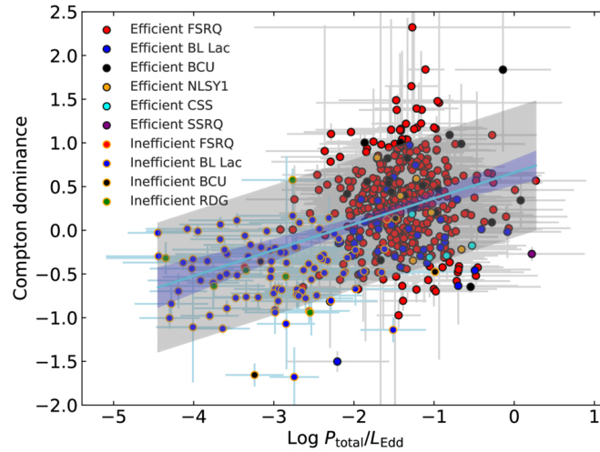
(d) jet power (normalized by Eddington luminosity) versus Compton dominance
