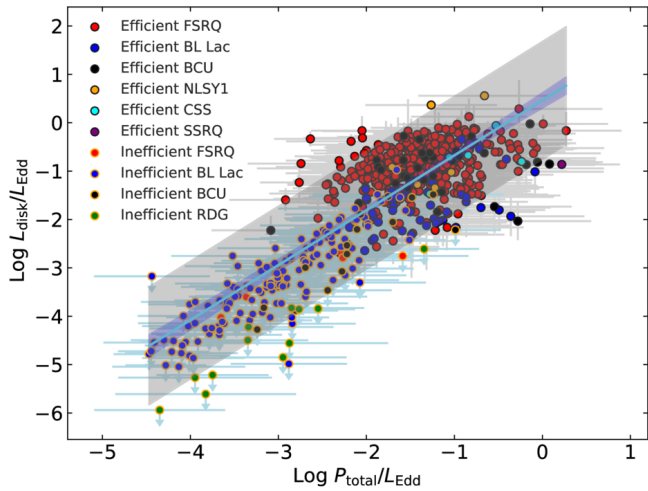
(c) jet power (normalized by Eddington luminosity) versus Eddington ratio
