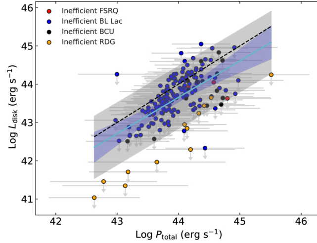
(b) Total jet power versus accretion disk luminosity in radiatively inefficient AGNs.
