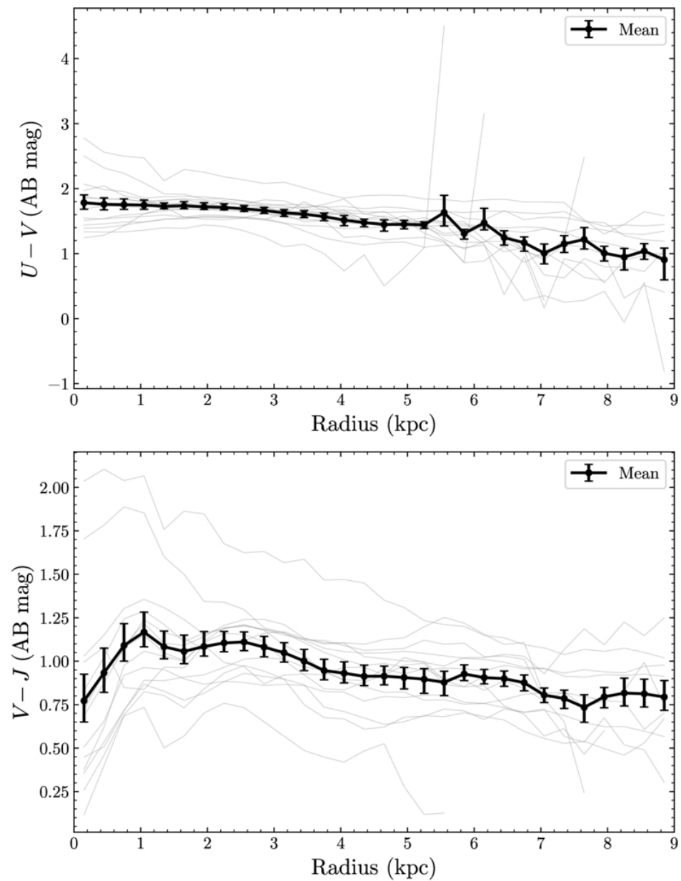
Figure 9. from Vaidik Prasal et al 2026 Astrophys. J. 1009 doi:10.3847/1538-4357/ae9a85 https://dx.doi.org/10.3847/1538-4357/ae9a85 © 2026. The Author(s). Published by the American Astronomical Society.
