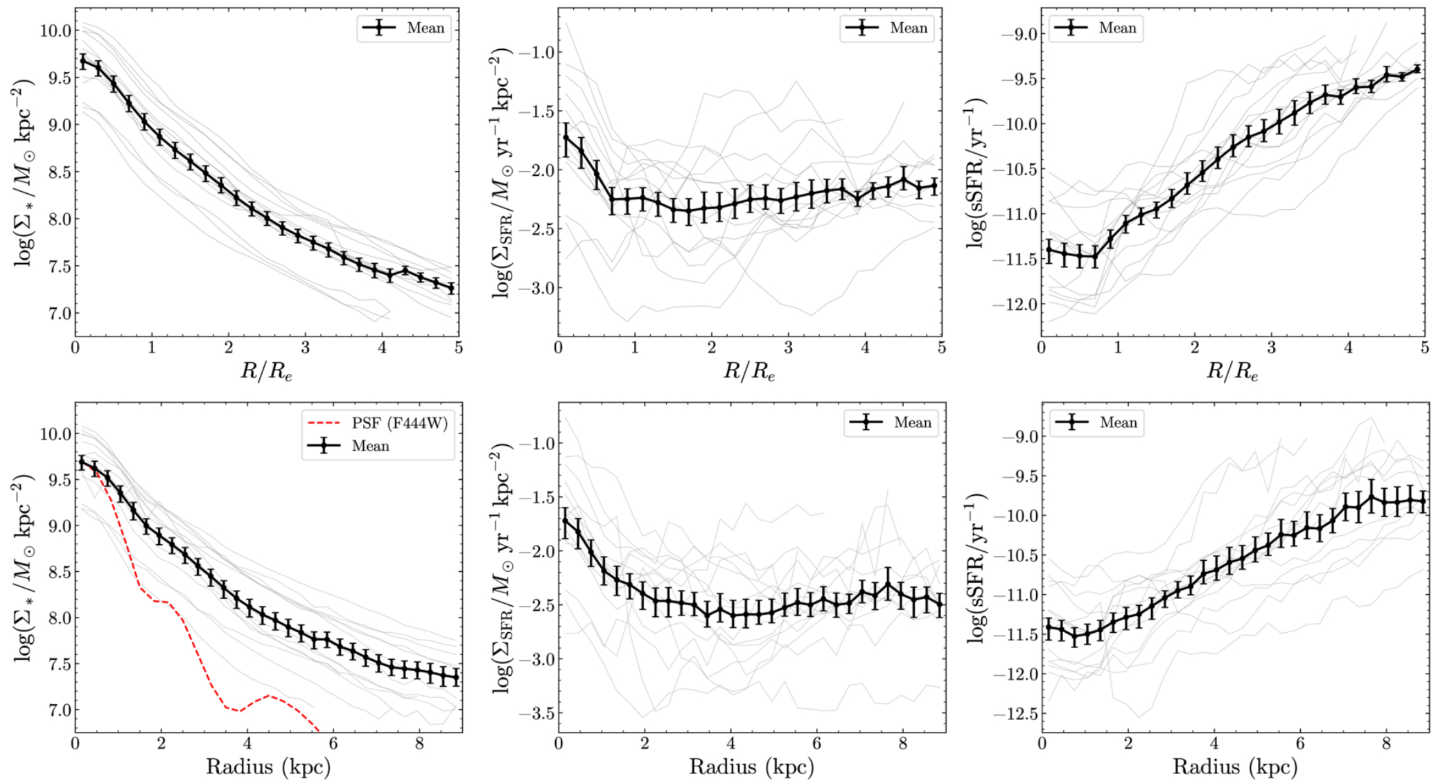
Figure 8. from Vaidik Prasal et al 2026 Astrophys. J. 1009 doi:10.3847/1538-4357/ae9a85 https://dx.doi.org/10.3847/1538-4357/ae9a85 © 2026. The Author(s). Published by the American Astronomical Society.
