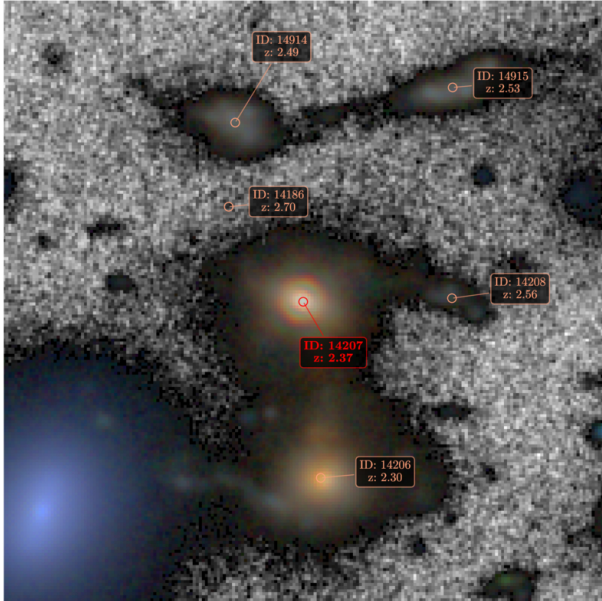
Figure 6. from Vaidik Prasal et al 2026 Astrophys. J. 1009 doi:10.3847/1538-4357/ae9a85 https://dx.doi.org/10.3847/1538-4357/ae9a85 © 2026. The Author(s). Published by the American Astronomical Society.
