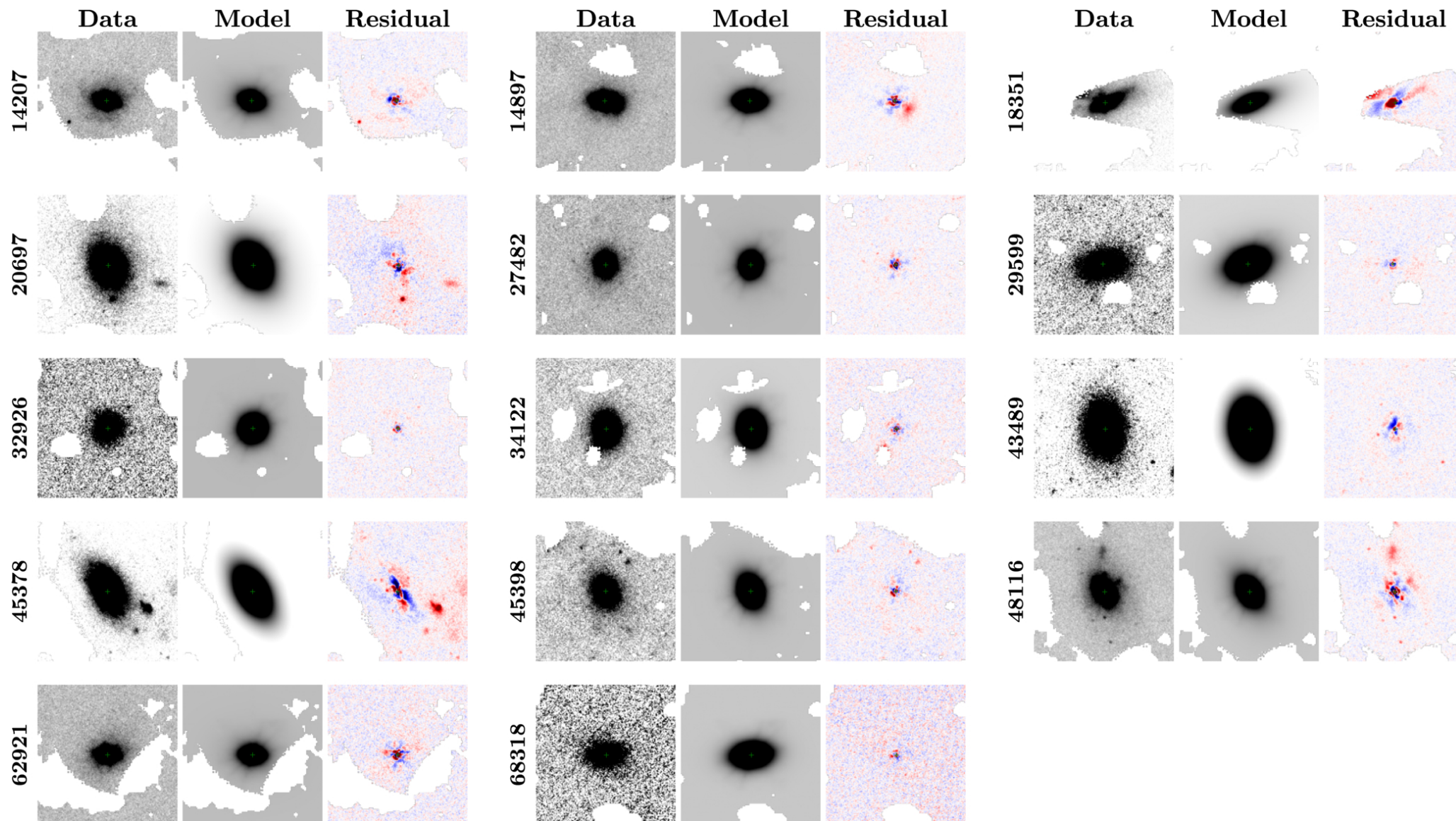
Figure 4. from Vaidik Prasal et al 2026 Astrophys. J. 1009 doi:10.3847/1538-4357/ae9a85 https://dx.doi.org/10.3847/1538-4357/ae9a85 © 2026. The Author(s). Published by the American Astronomical Society.
