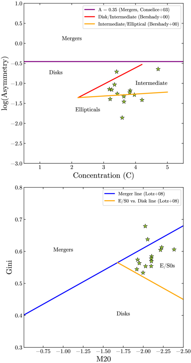
Figure 3. from Vaidik Prasal et al 2026 Astrophys. J. 1009 doi:10.3847/1538-4357/ae9a85 https://dx.doi.org/10.3847/1538-4357/ae9a85 © 2026. The Author(s). Published by the American Astronomical Society.
