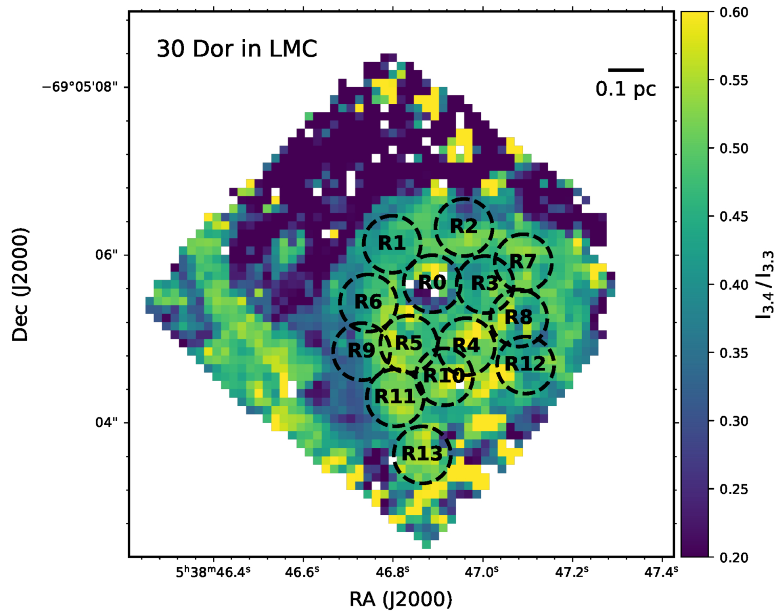
Figure 6. from Junhao Peng et al 2026 Astrophys. J. 1010 doi:10.3847/1538-4357/ae9a80 https://dx.doi.org/10.3847/1538-4357/ae9a80 © 2026. The Author(s). Published by the American Astronomical Society.
