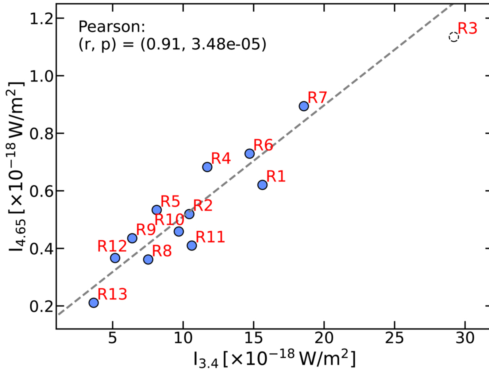
Figure 10. from Junhao Peng et al 2026 Astrophys. J. 1010 doi:10.3847/1538-4357/ae9a80 https://dx.doi.org/10.3847/1538-4357/ae9a80 © 2026. The Author(s). Published by the American Astronomical Society.
