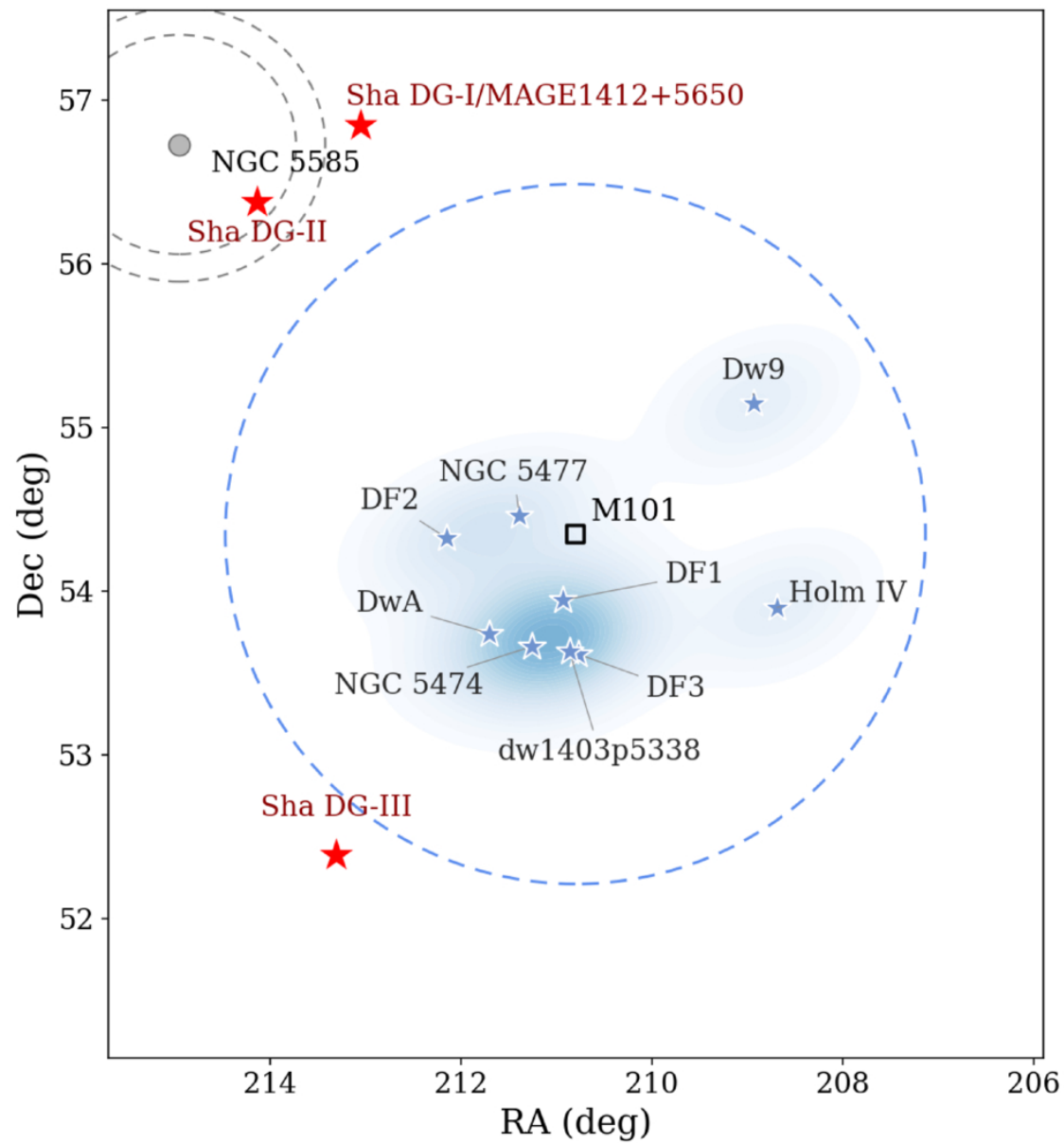
Figure 2. from Julian Shapiro 2026 Astrophys. J. 1010 doi:10.3847/1538-4357/ae99cb https://dx.doi.org/10.3847/1538-4357/ae99cb © 2026. The Author(s). Published by the American Astronomical Society.
