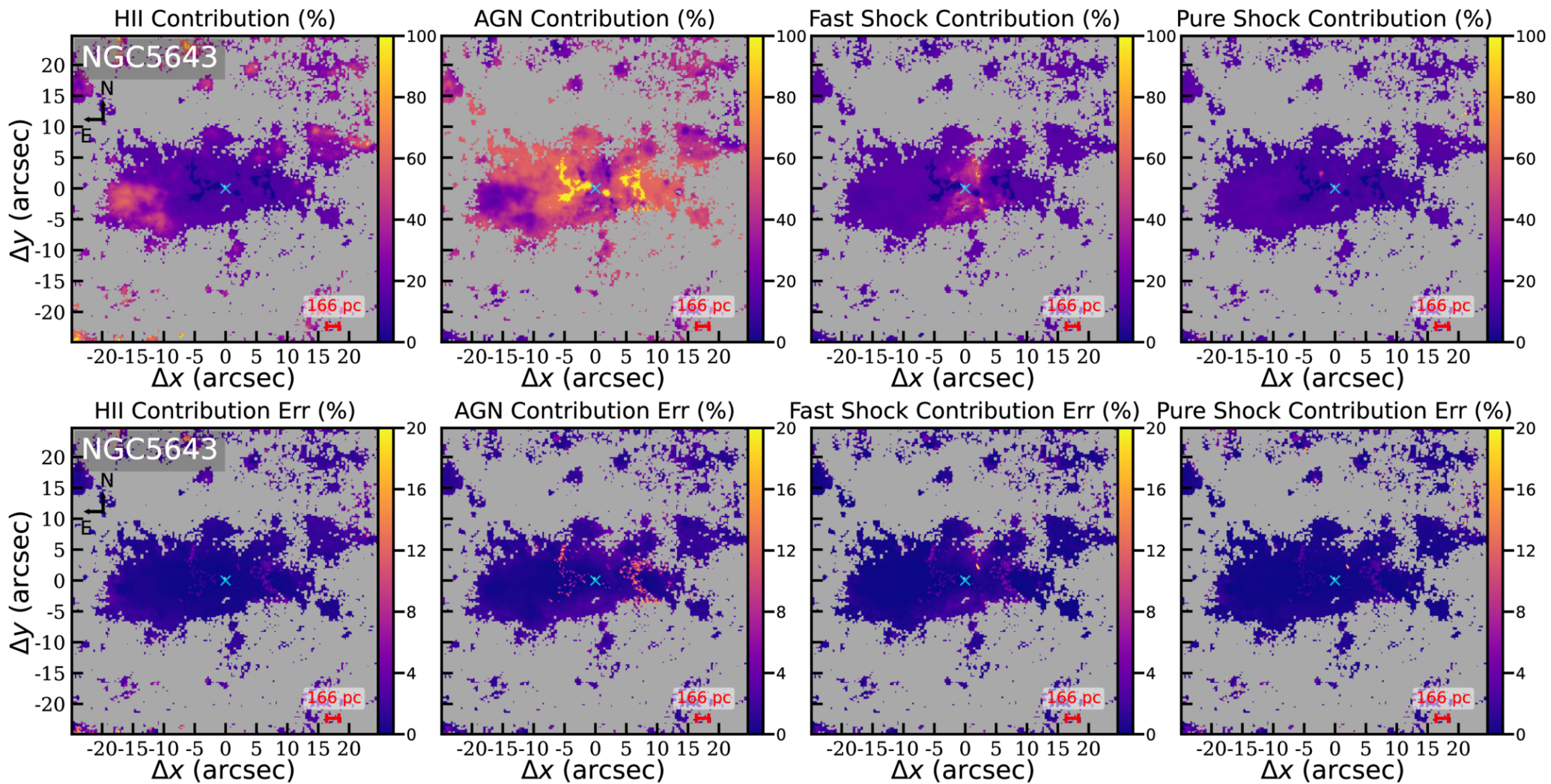
Figure 8. from Peixin Zhu et al 2026 Astrophys. J. 1009 doi:10.3847/1538-4357/ae9956 https://dx.doi.org/10.3847/1538-4357/ae9956 © 2026. The Author(s). Published by the American Astronomical Society.
