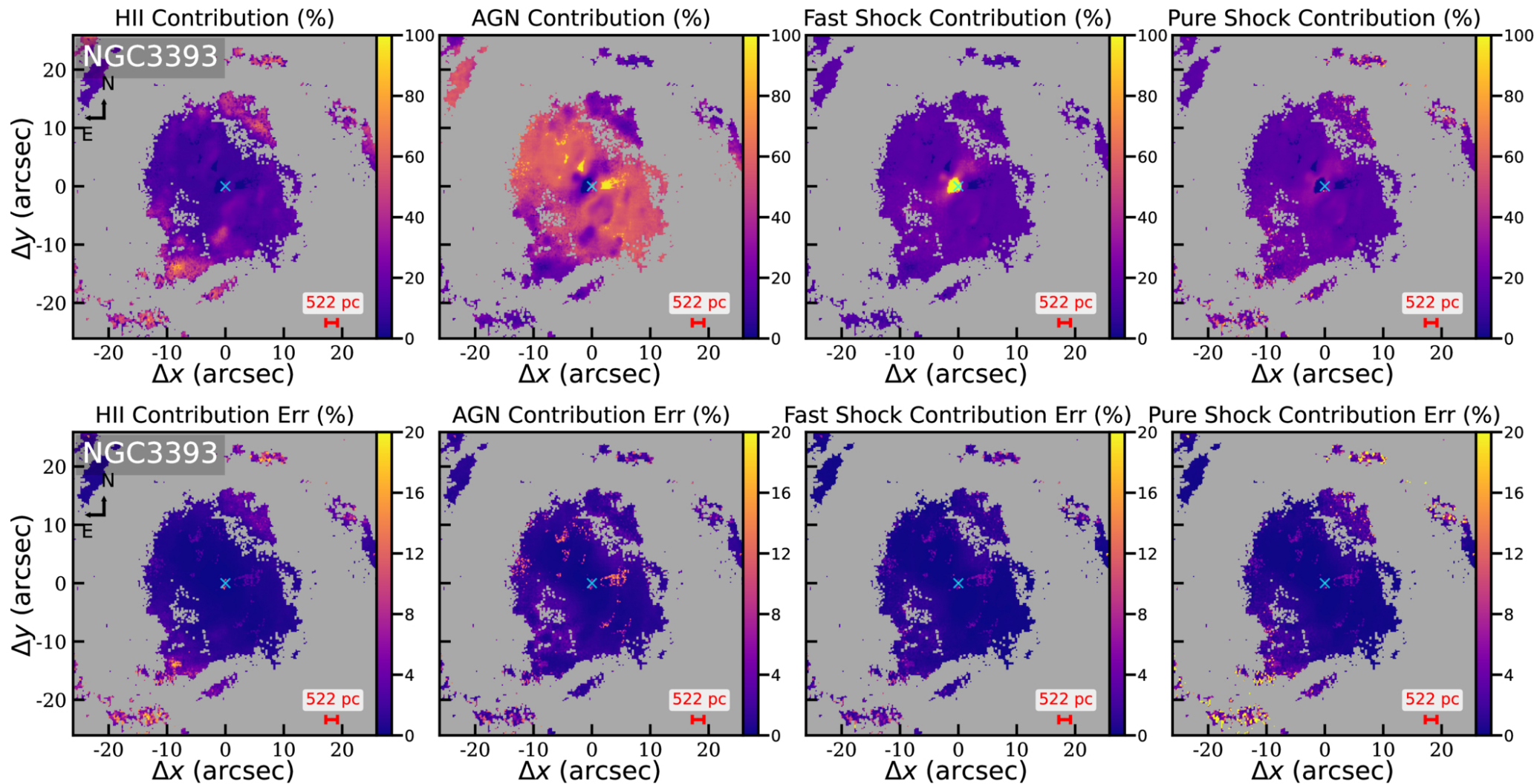
Figure 7. from Peixin Zhu et al 2026 Astrophys. J. 1009 doi:10.3847/1538-4357/ae9956 https://dx.doi.org/10.3847/1538-4357/ae9956 © 2026. The Author(s). Published by the American Astronomical Society.
