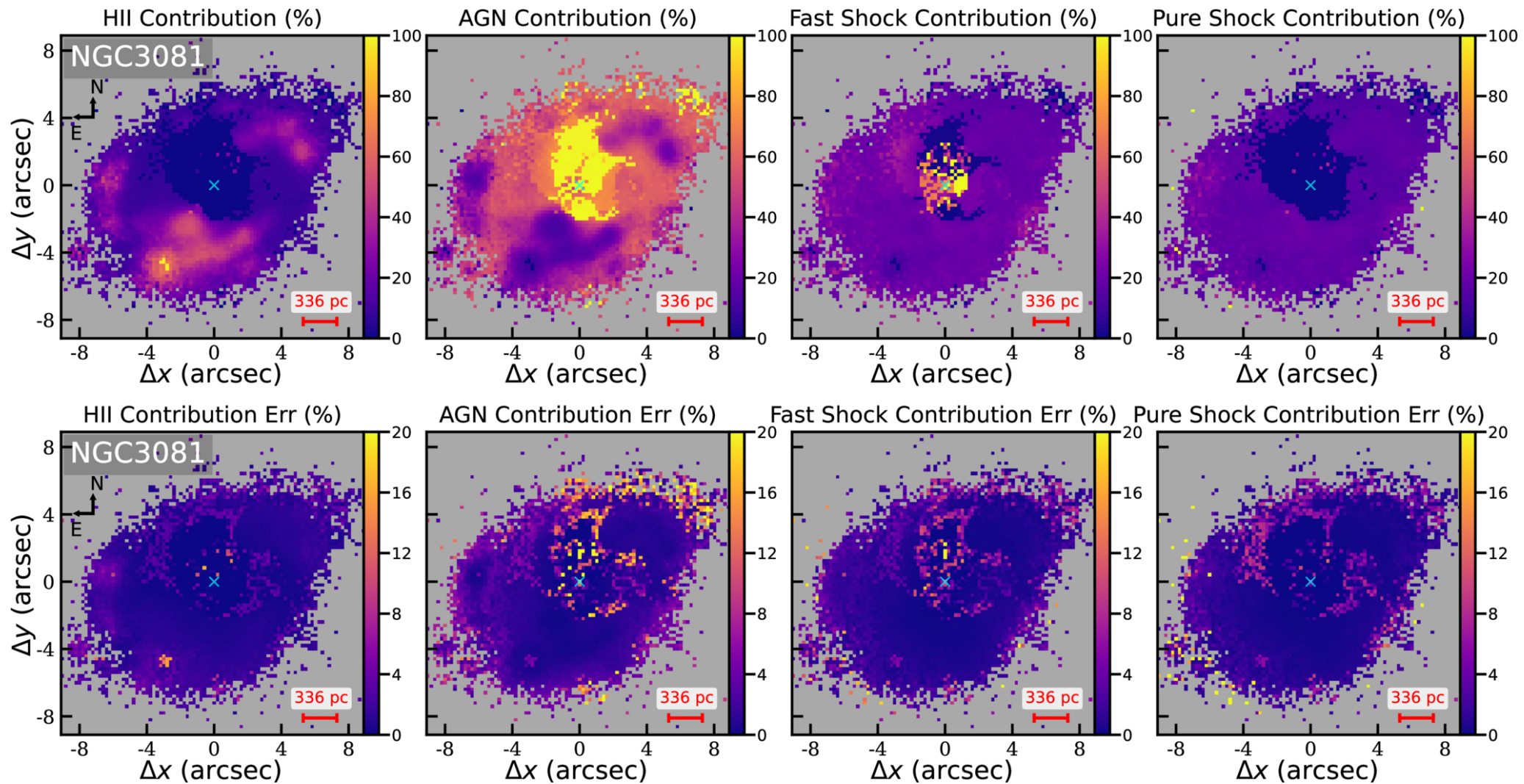
Figure 6. from Peixin Zhu et al 2026 Astrophys. J. 1009 doi:10.3847/1538-4357/ae9956 https://dx.doi.org/10.3847/1538-4357/ae9956 © 2026. The Author(s). Published by the American Astronomical Society.
