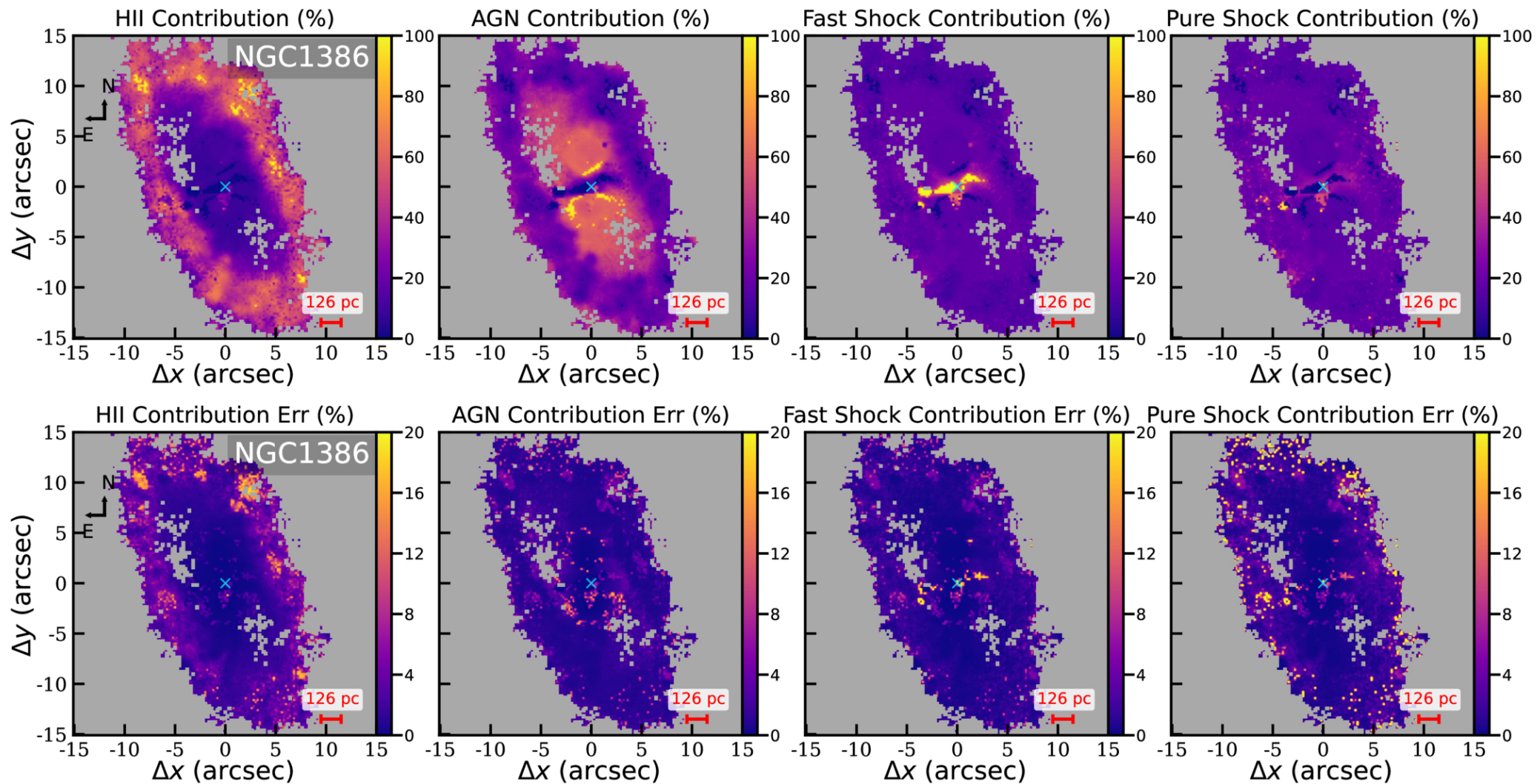
Figure 5. from Peixin Zhu et al 2026 Astrophys. J. 1009 doi:10.3847/1538-4357/ae9956 https://dx.doi.org/10.3847/1538-4357/ae9956 © 2026. The Author(s). Published by the American Astronomical Society.
