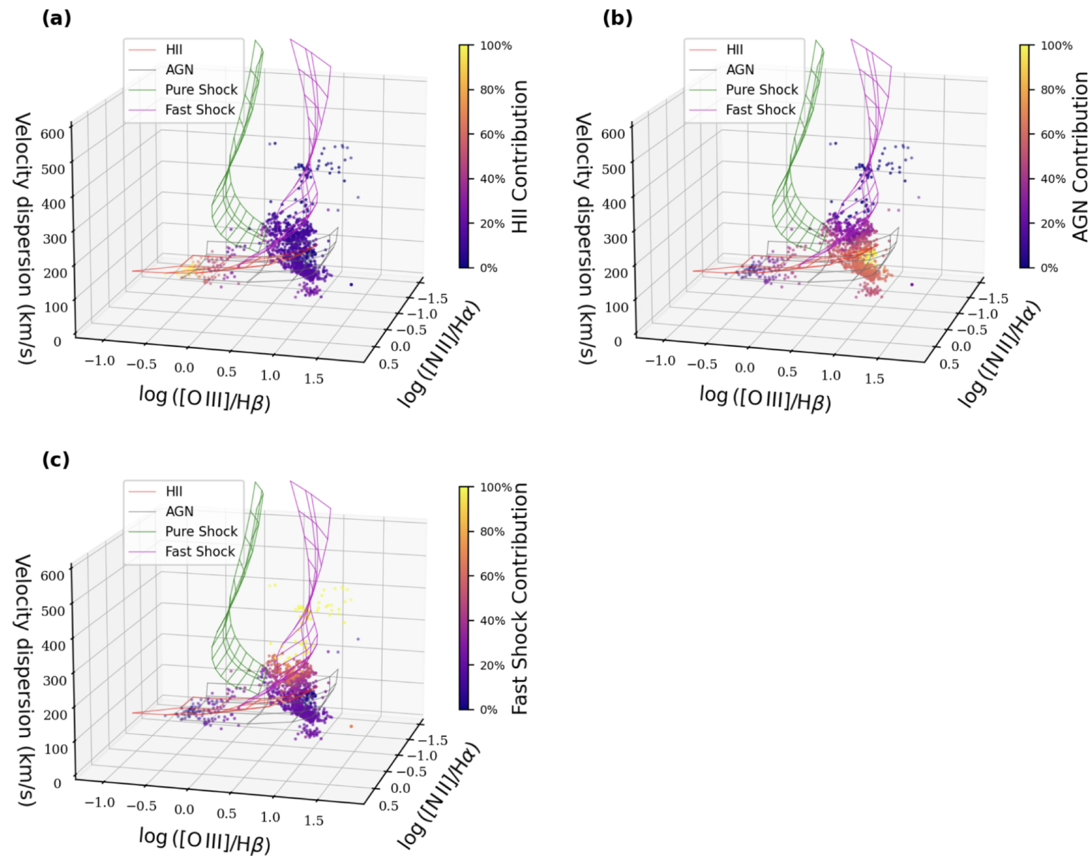
Figure A7. from Peixin Zhu et al 2026 Astrophys. J. 1009 doi:10.3847/1538-4357/ae9956 https://dx.doi.org/10.3847/1538-4357/ae9956 © 2026. The Author(s). Published by the American Astronomical Society.
