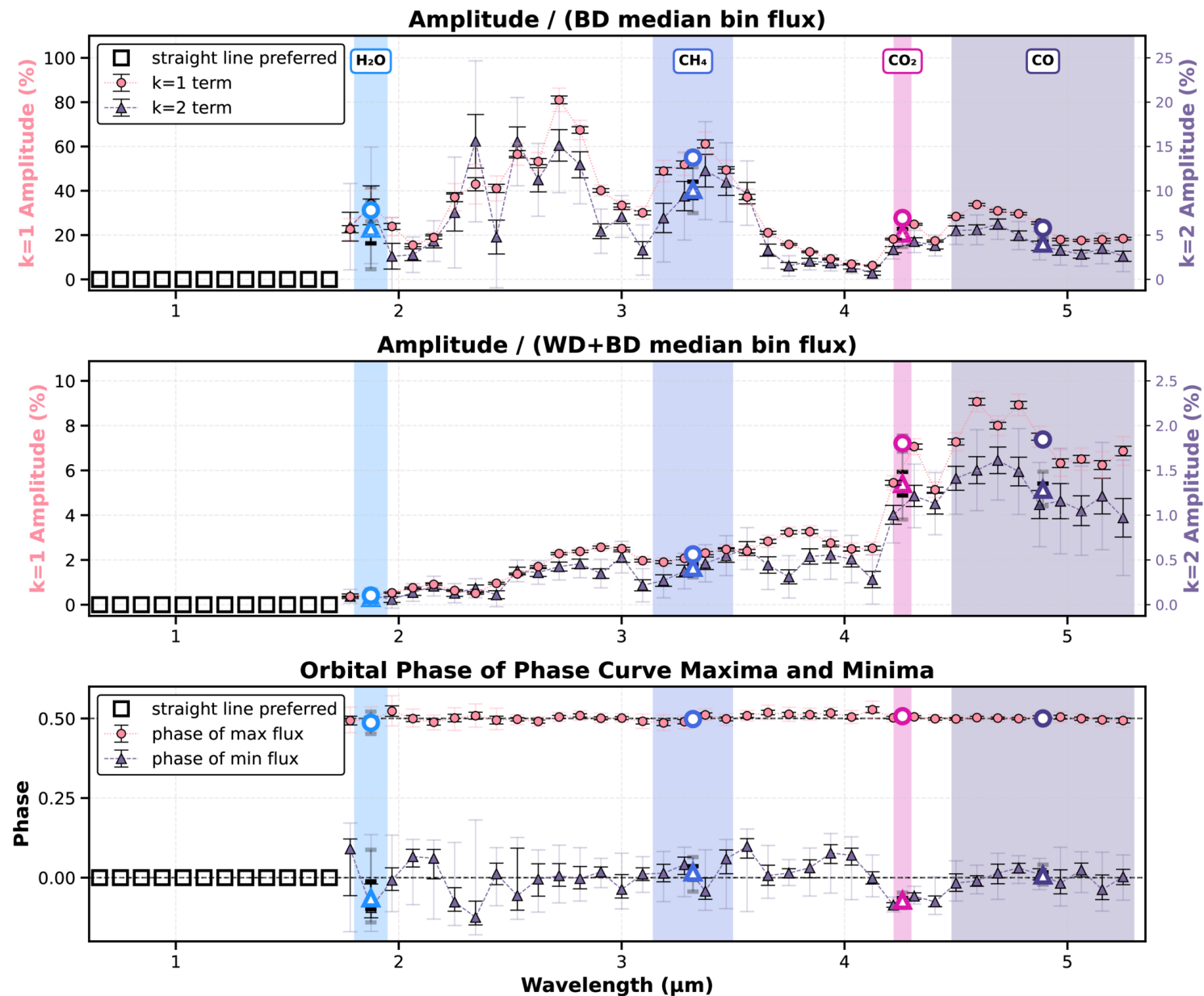
Figure 7. from Daphne Broski-Laing et al 2026 Astrophys. J. 1009 doi:10.3847/1538-4357/ae9940 https://dx.doi.org/10.3847/1538-4357/ae9940 © 2026. The Author(s). Published by the American Astronomical Society.
