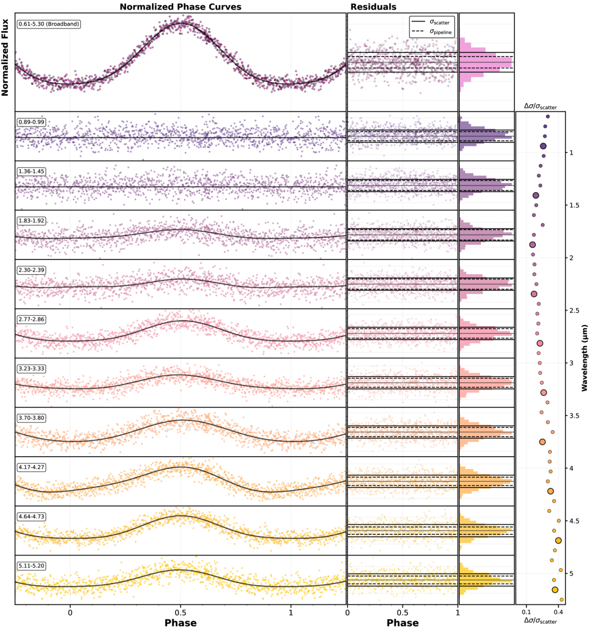
Figure 4. from Daphne Broski-Laing et al 2026 Astrophys. J. 1009 doi:10.3847/1538-4357/ae9940 https://dx.doi.org/10.3847/1538-4357/ae9940 © 2026. The Author(s). Published by the American Astronomical Society.
