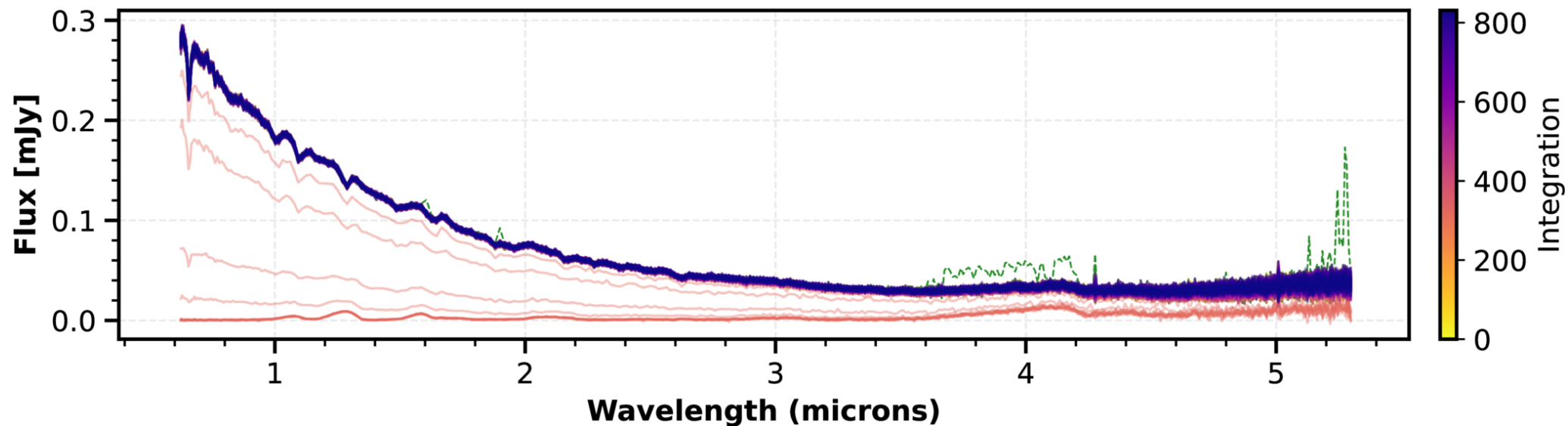
Figure 2. from Daphne Broski-Laing et al 2026 Astrophys. J. 1009 doi:10.3847/1538-4357/ae9940 https://dx.doi.org/10.3847/1538-4357/ae9940 © 2026. The Author(s). Published by the American Astronomical Society.
