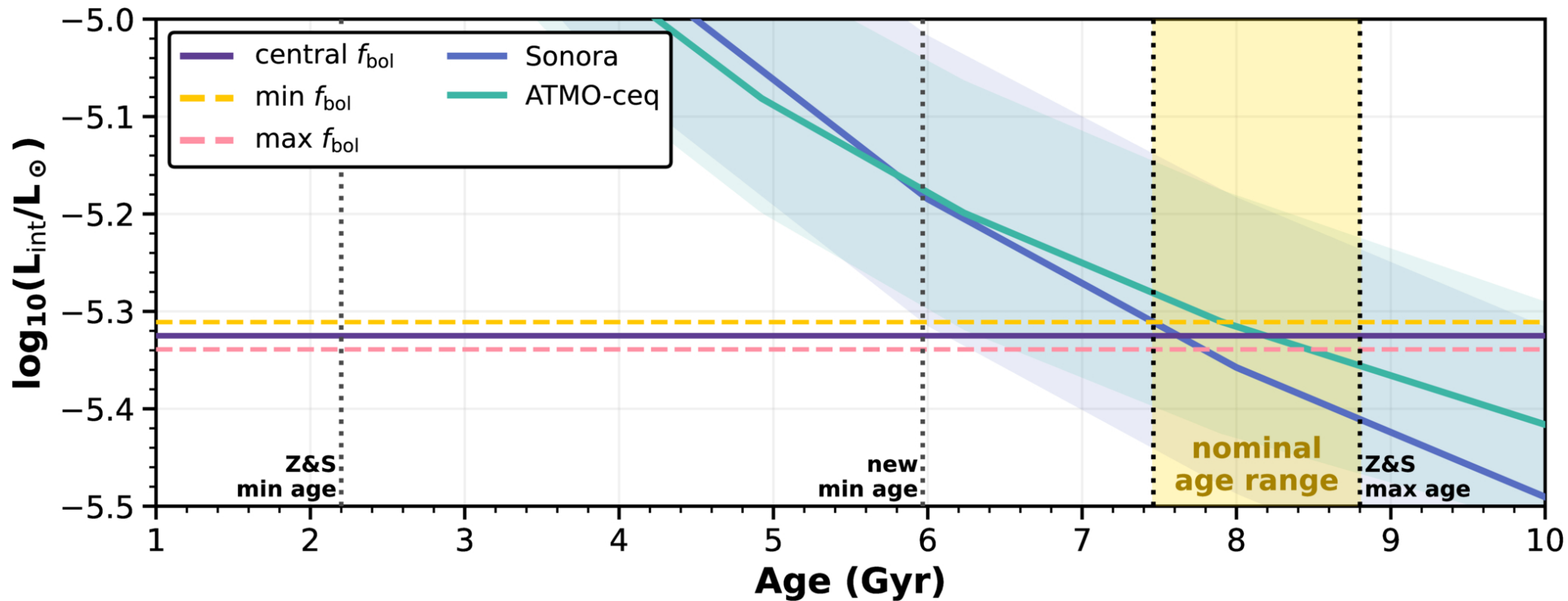
Figure 19. from Daphne Broski-Laing et al 2026 Astrophys. J. 1009 doi:10.3847/1538-4357/ae9940 https://dx.doi.org/10.3847/1538-4357/ae9940 © 2026. The Author(s). Published by the American Astronomical Society.
