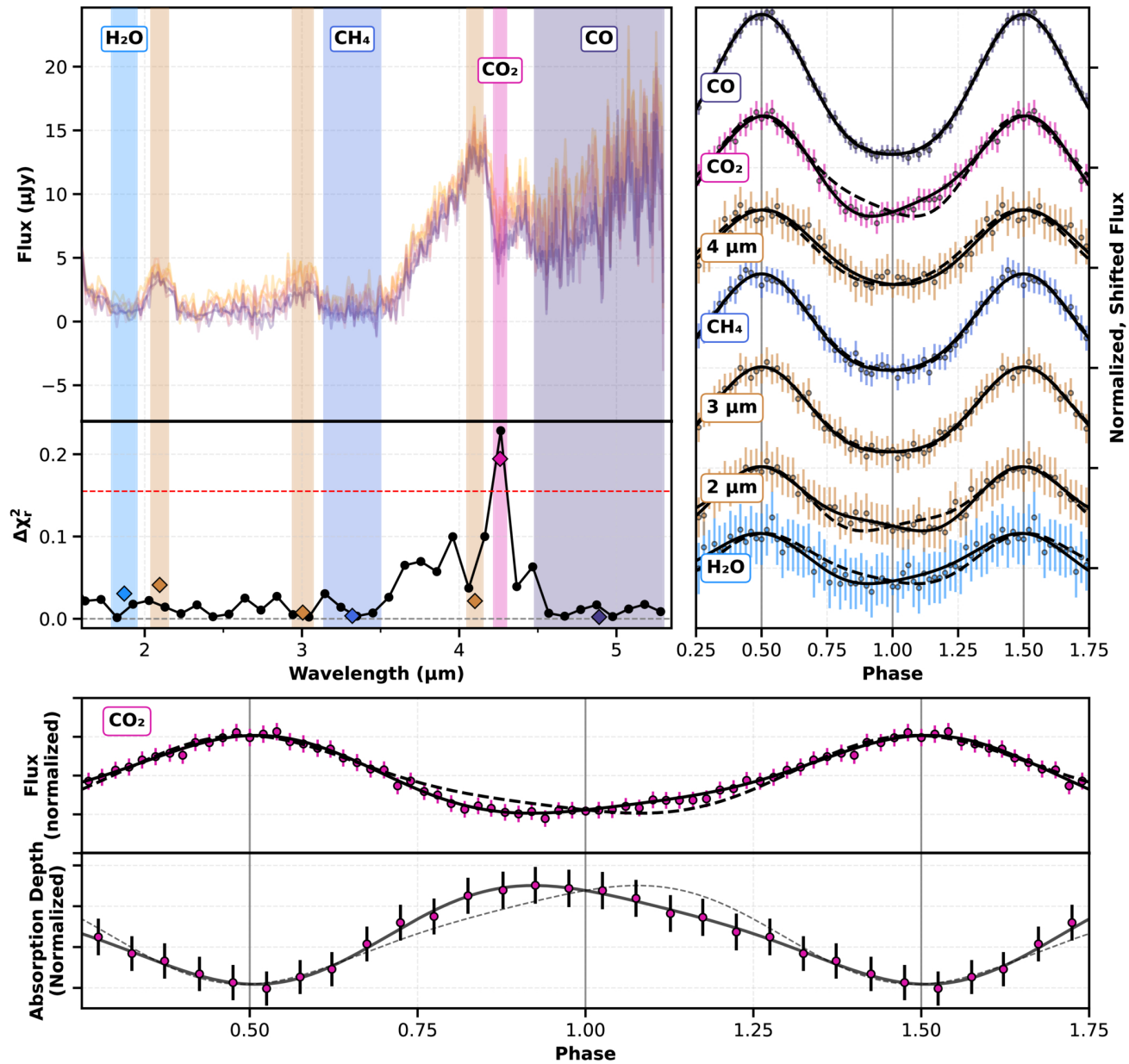
Figure 16. from Daphne Broski-Laing et al 2026 Astrophys. J. 1009 doi:10.3847/1538-4357/ae9940 https://dx.doi.org/10.3847/1538-4357/ae9940 © 2026. The Author(s). Published by the American Astronomical Society.
