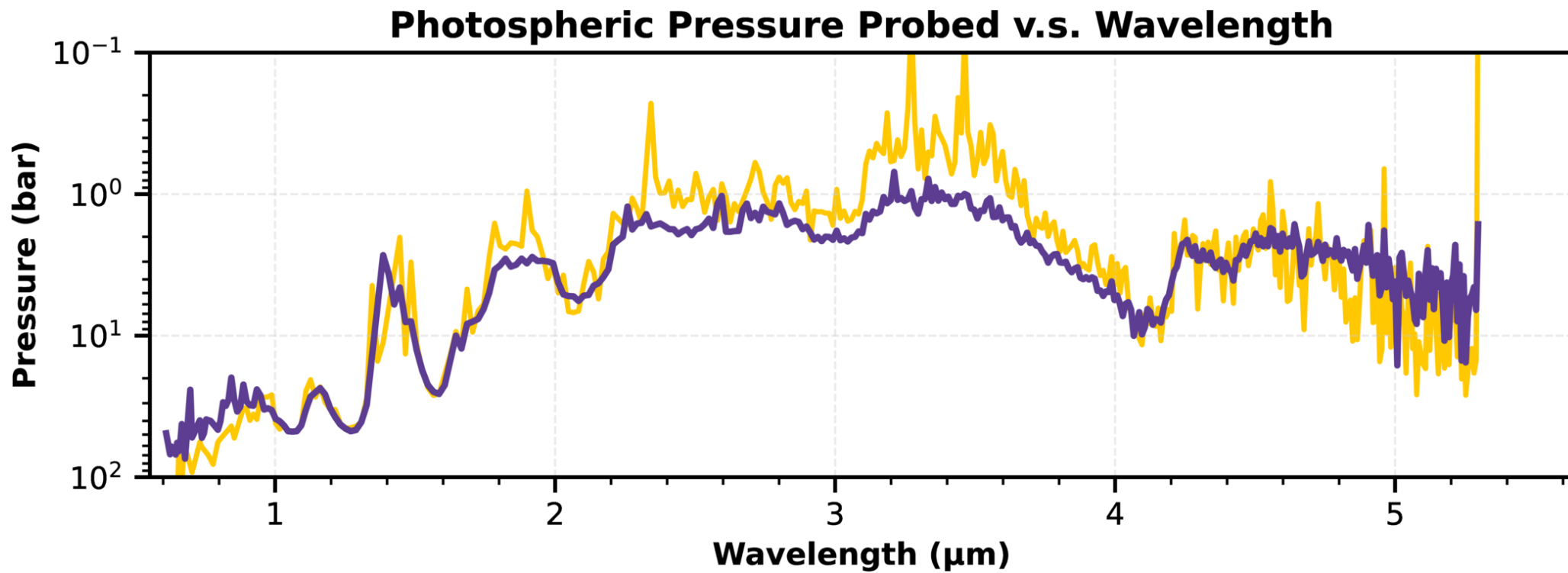
Figure 14. from Daphne Broski-Laing et al 2026 Astrophys. J. 1009 doi:10.3847/1538-4357/ae9940 https://dx.doi.org/10.3847/1538-4357/ae9940 © 2026. The Author(s). Published by the American Astronomical Society.
