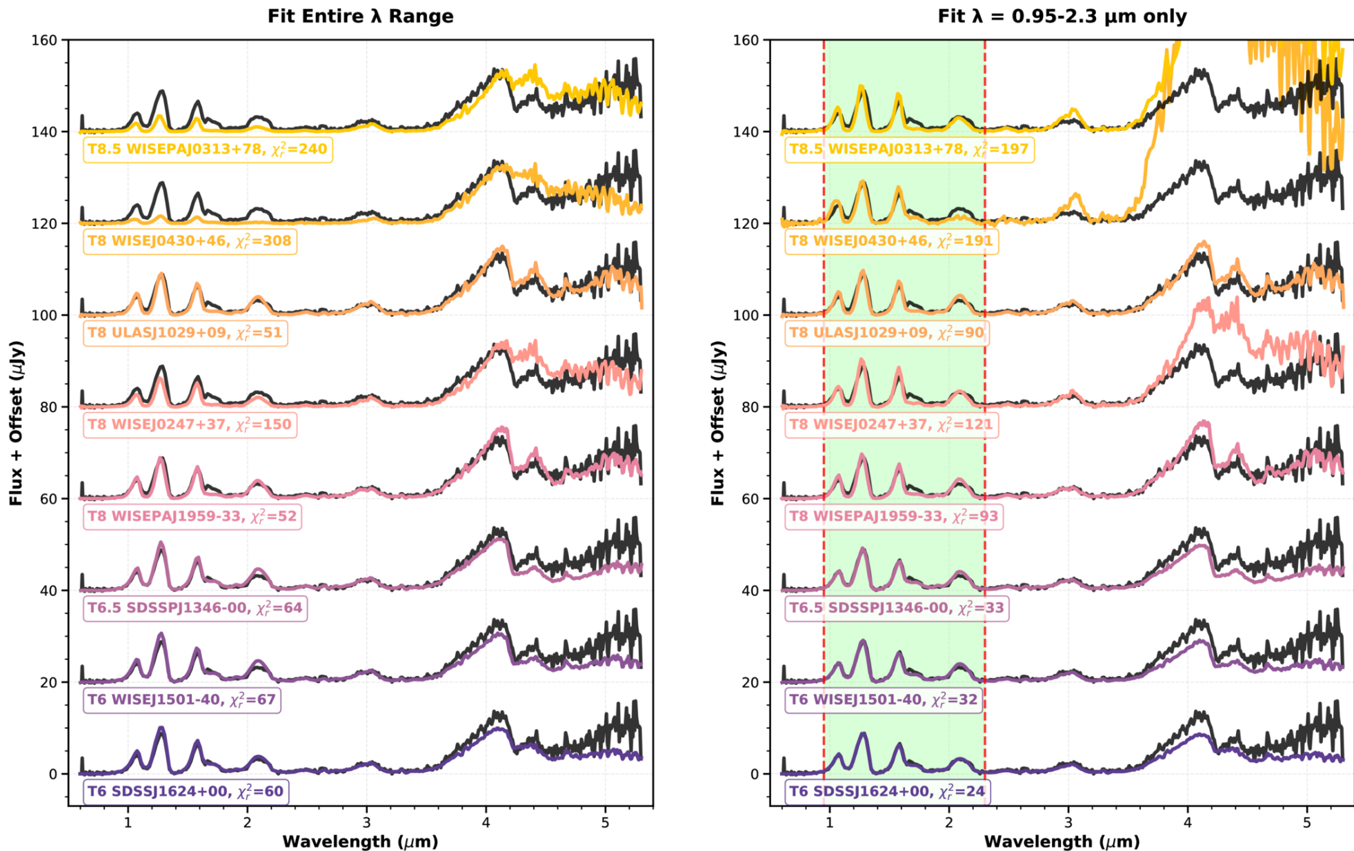
Figure 10. from Daphne Broski-Laing et al 2026 Astrophys. J. 1009 doi:10.3847/1538-4357/ae9940 https://dx.doi.org/10.3847/1538-4357/ae9940 © 2026. The Author(s). Published by the American Astronomical Society.
