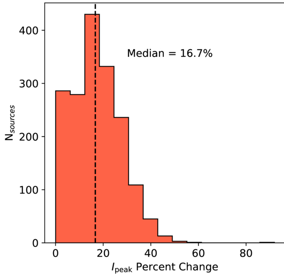
Figure B1. from Jennifer Wallace et al 2026 Astrophys. J. 1009 doi:10.3847/1538-4357/ae990d https://dx.doi.org/10.3847/1538-4357/ae990d © 2026. The Author(s). Published by the American Astronomical Society.
