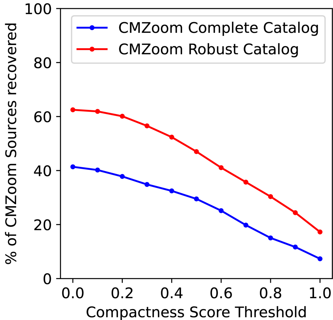
Figure 7. from Jennifer Wallace et al 2026 Astrophys. J. 1009 doi:10.3847/1538-4357/ae990d https://dx.doi.org/10.3847/1538-4357/ae990d © 2026. The Author(s). Published by the American Astronomical Society.
