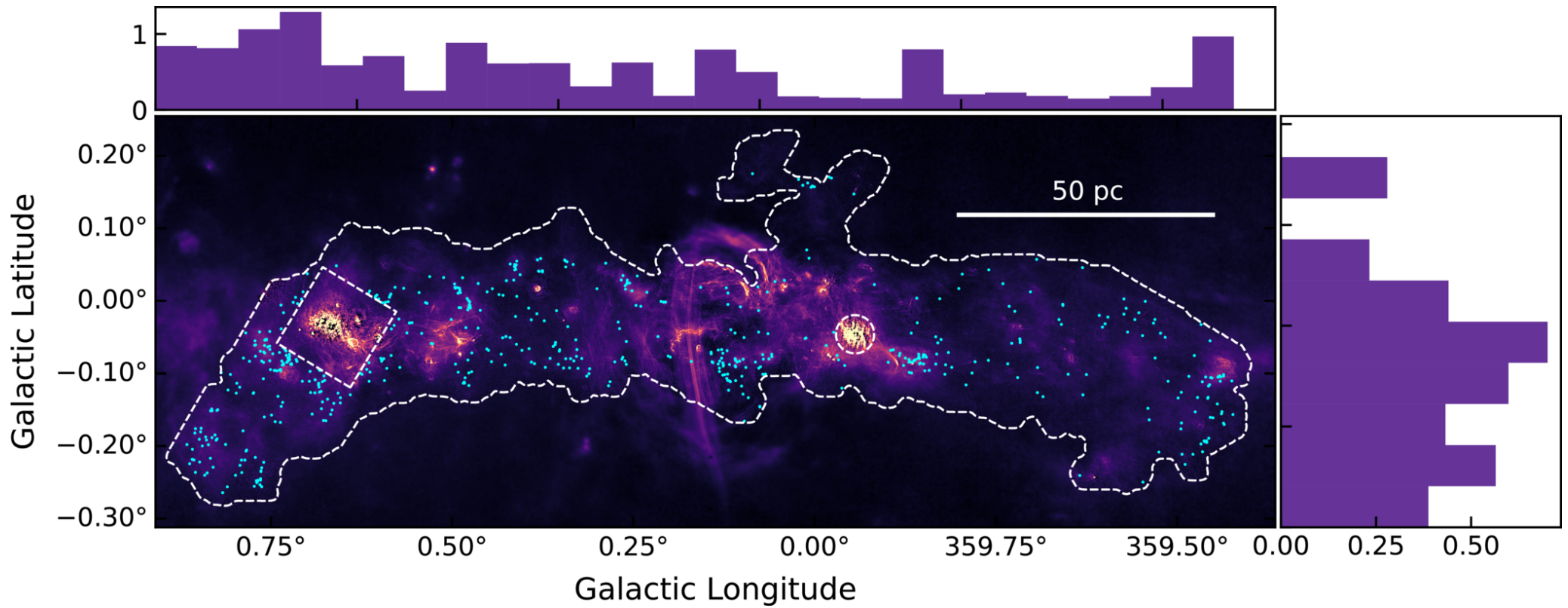
Figure 6. from Jennifer Wallace et al 2026 Astrophys. J. 1009 doi:10.3847/1538-4357/ae990d https://dx.doi.org/10.3847/1538-4357/ae990d © 2026. The Author(s). Published by the American Astronomical Society.
