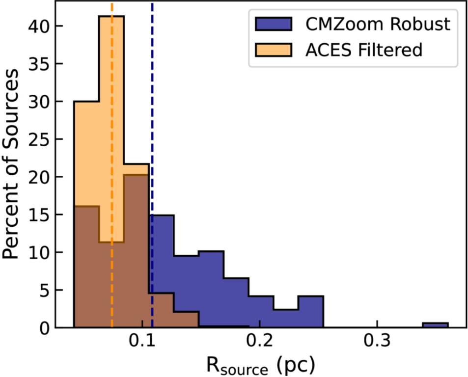
Figure 5. from Jennifer Wallace et al 2026 Astrophys. J. 1009 doi:10.3847/1538-4357/ae990d https://dx.doi.org/10.3847/1538-4357/ae990d © 2026. The Author(s). Published by the American Astronomical Society.
