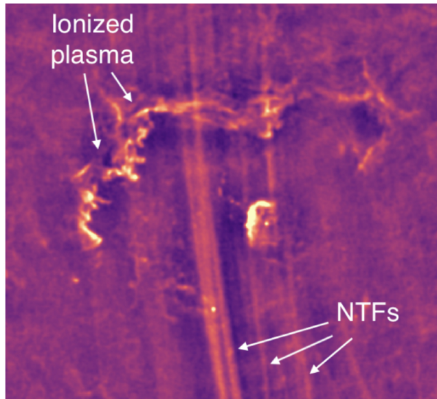
Figure 3. Zooniverse Tutorial from Jennifer Wallace et al 2026 Astrophys. J. 1009 doi:10.3847/1538-4357/ae990d https://dx.doi.org/10.3847/1538-4357/ae990d © 2026. The Author(s). Published by the American Astronomical Society.
