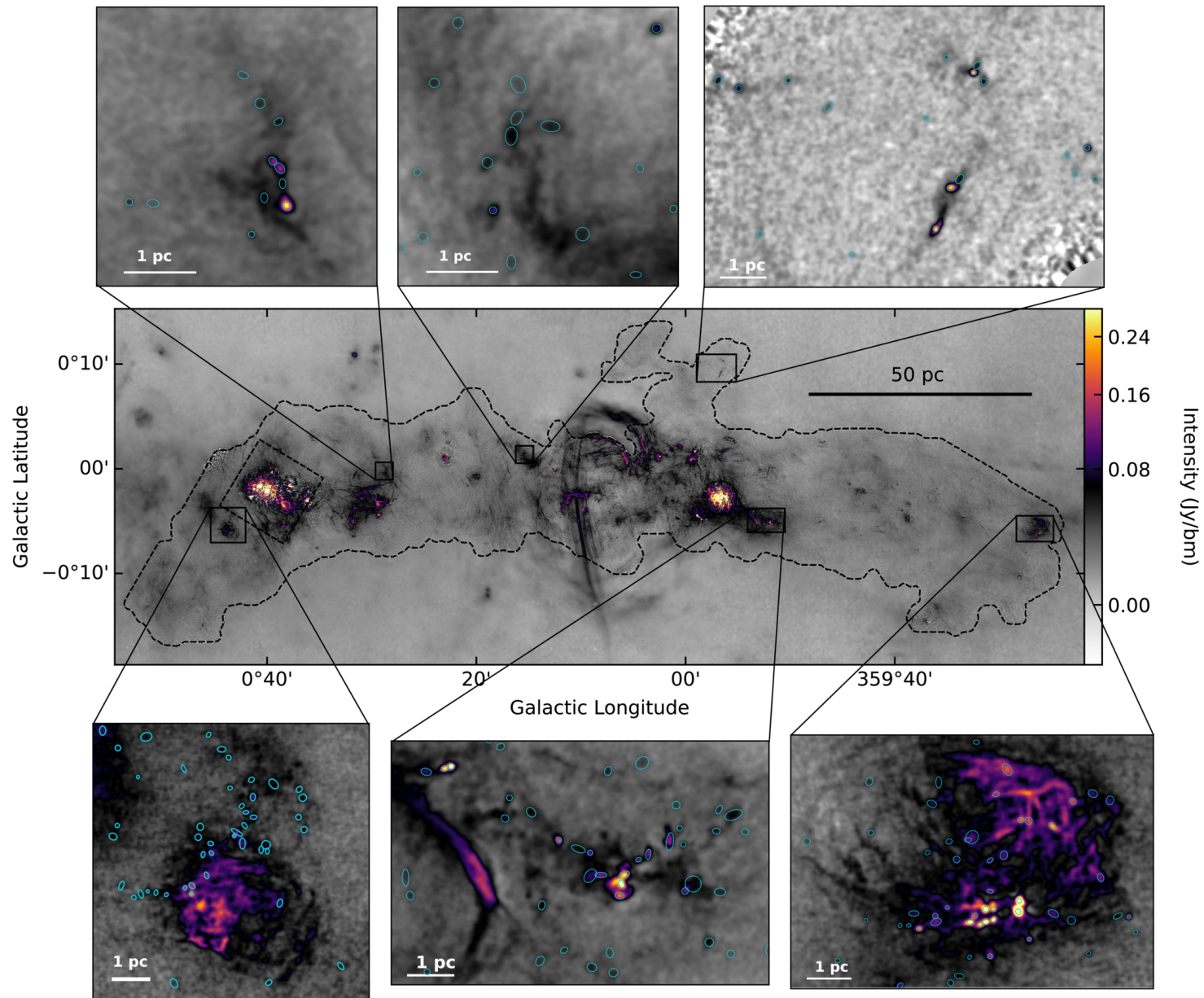
Figure 1. from Jennifer Wallace et al 2026 Astrophys. J. 1009 doi:10.3847/1538-4357/ae990d https://dx.doi.org/10.3847/1538-4357/ae990d © 2026. The Author(s). Published by the American Astronomical Society.
