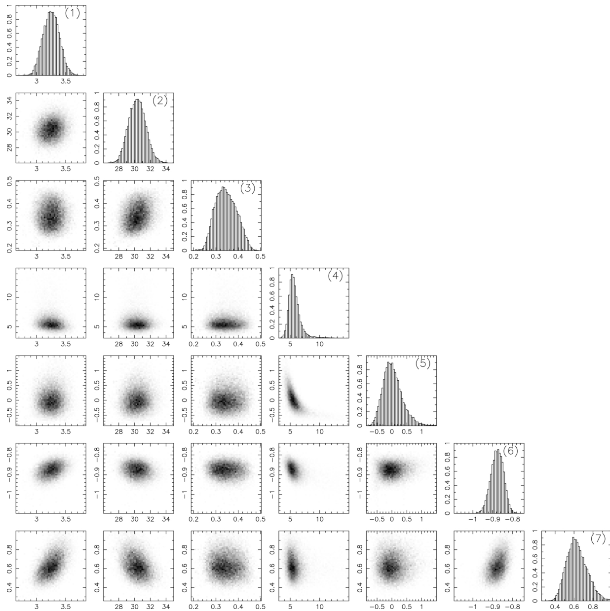
Figure 8. from David Nesvorný et al 2026 Astrophys. J. 1008 doi:10.3847/1538-4357/ae9870 https://dx.doi.org/10.3847/1538-4357/ae9870 © 2026. The Author(s). Published by the American Astronomical Society.
