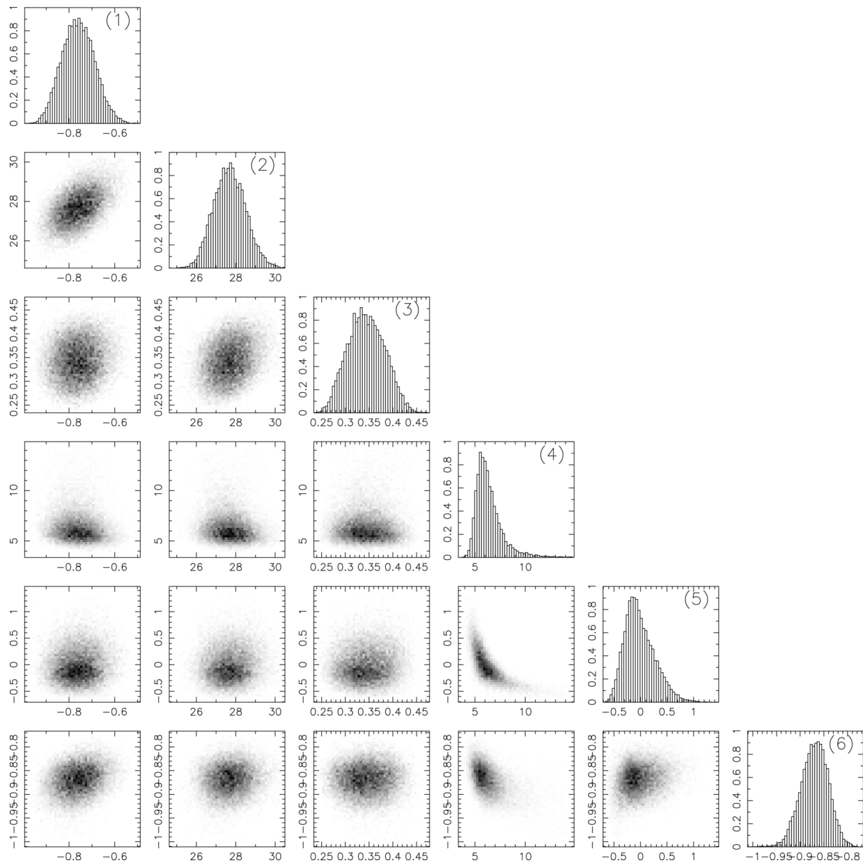
Figure 7. from David Nesvorný et al 2026 Astrophys. J. 1008 doi:10.3847/1538-4357/ae9870 https://dx.doi.org/10.3847/1538-4357/ae9870 © 2026. The Author(s). Published by the American Astronomical Society.
