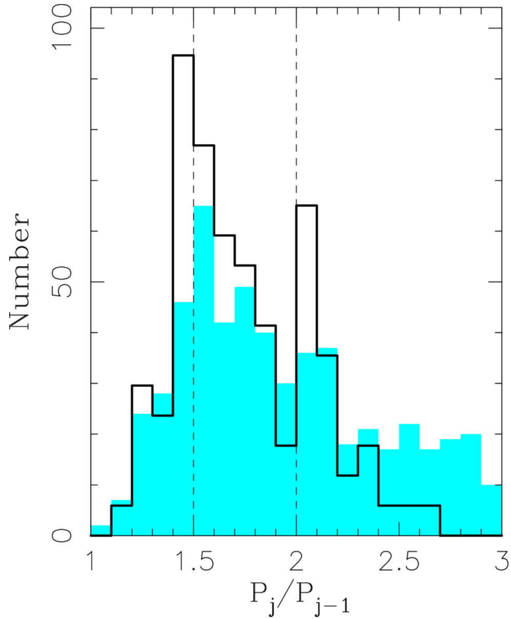
Figure 6. from David Nesvorný et al 2026 Astrophys. J. 1008 doi:10.3847/1538-4357/ae9870 https://dx.doi.org/10.3847/1538-4357/ae9870 © 2026. The Author(s). Published by the American Astronomical Society.
