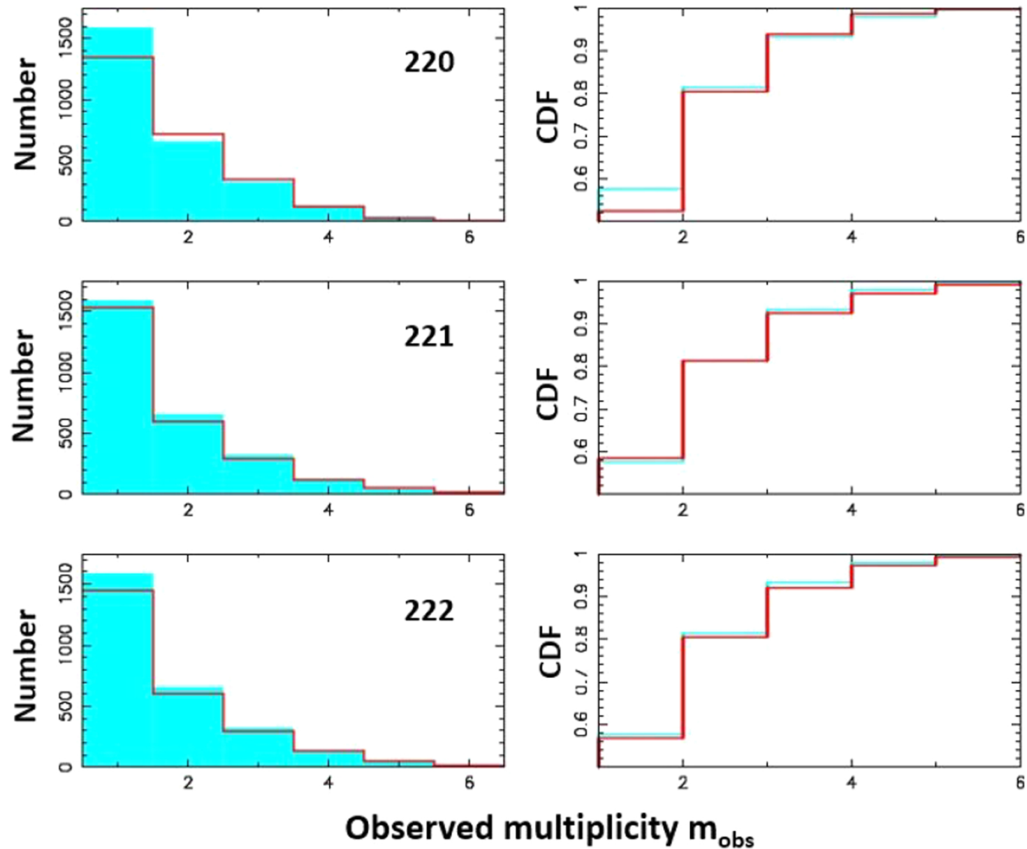
Figure 5. from David Nesvorný et al 2026 Astrophys. J. 1008 doi:10.3847/1538-4357/ae9870 https://dx.doi.org/10.3847/1538-4357/ae9870 © 2026. The Author(s). Published by the American Astronomical Society.
