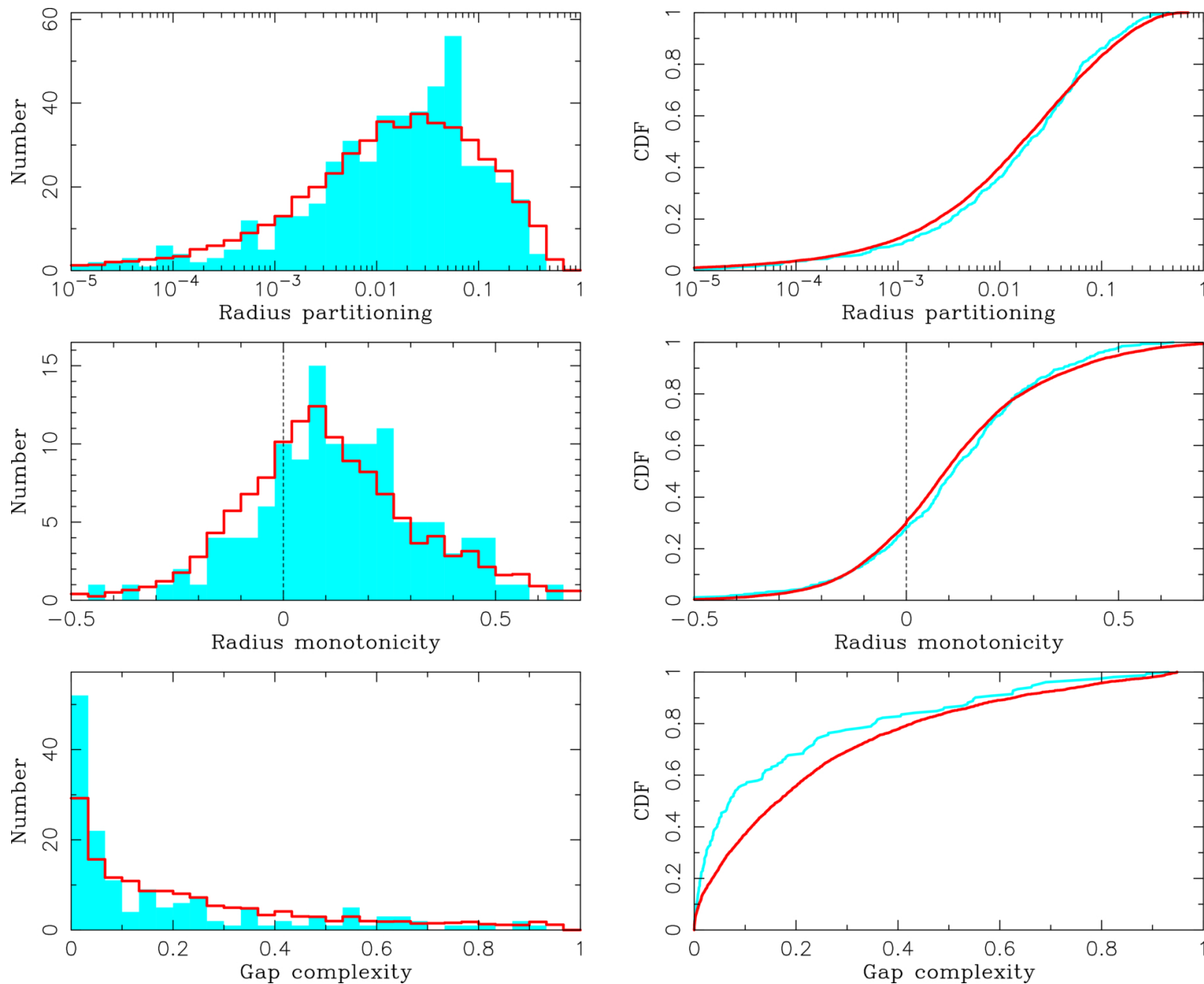
Figure 4. from David Nesvorný et al 2026 Astrophys. J. 1008 doi:10.3847/1538-4357/ae9870 https://dx.doi.org/10.3847/1538-4357/ae9870 © 2026. The Author(s). Published by the American Astronomical Society.
