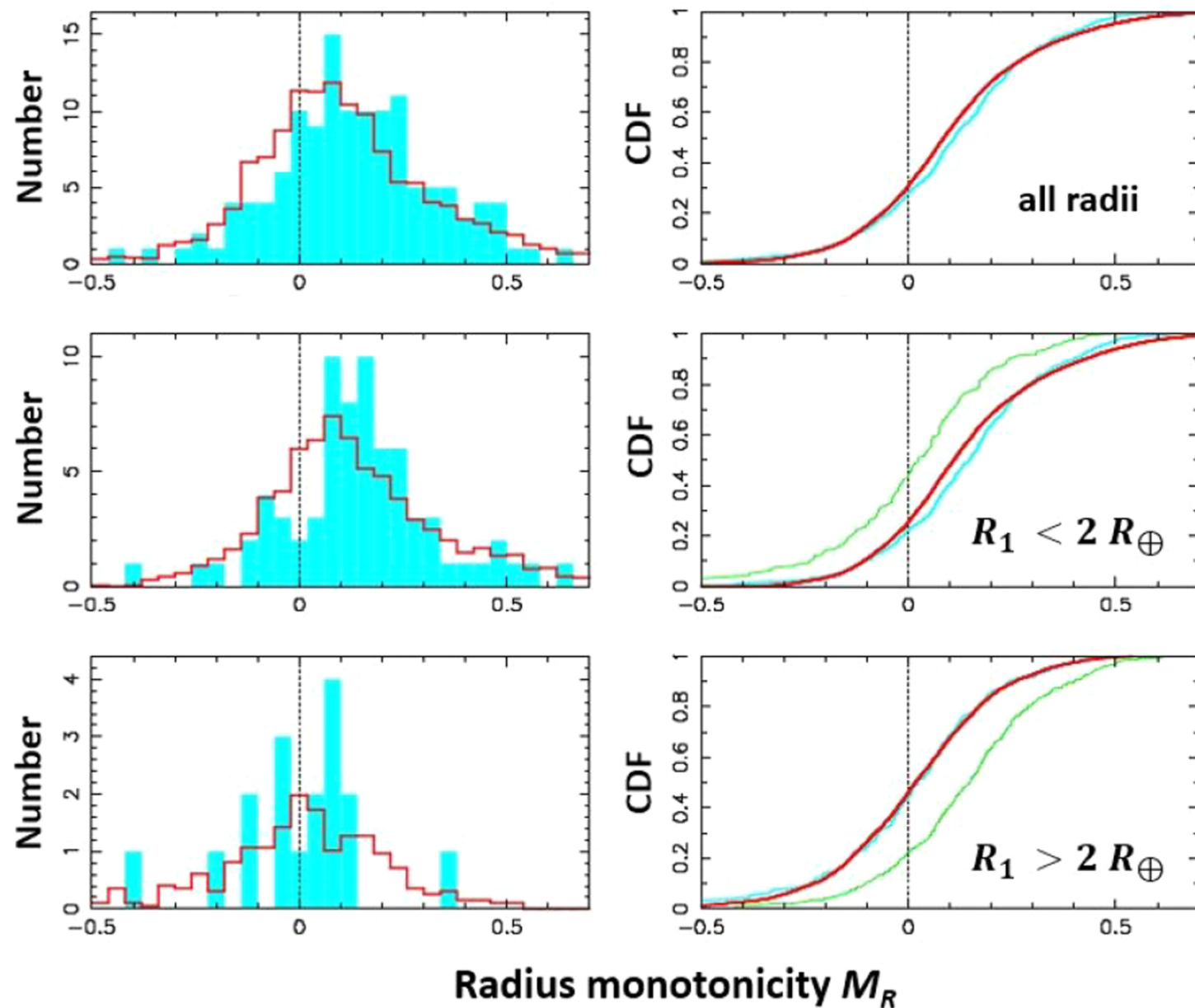
Figure 11. from David Nesvorný et al 2026 Astrophys. J. 1008 doi:10.3847/1538-4357/ae9870 https://dx.doi.org/10.3847/1538-4357/ae9870 © 2026. The Author(s). Published by the American Astronomical Society.
