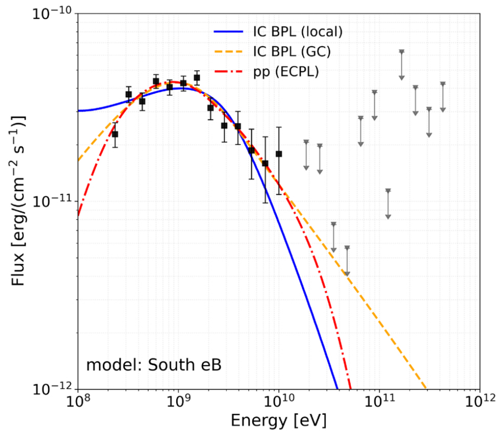
Figure B1. from Zhen Xie et al 2026 Astrophys. J. 1009 doi:10.3847/1538-4357/ae986d https://dx.doi.org/10.3847/1538-4357/ae986d © 2026. The Author(s). Published by the American Astronomical Society.
