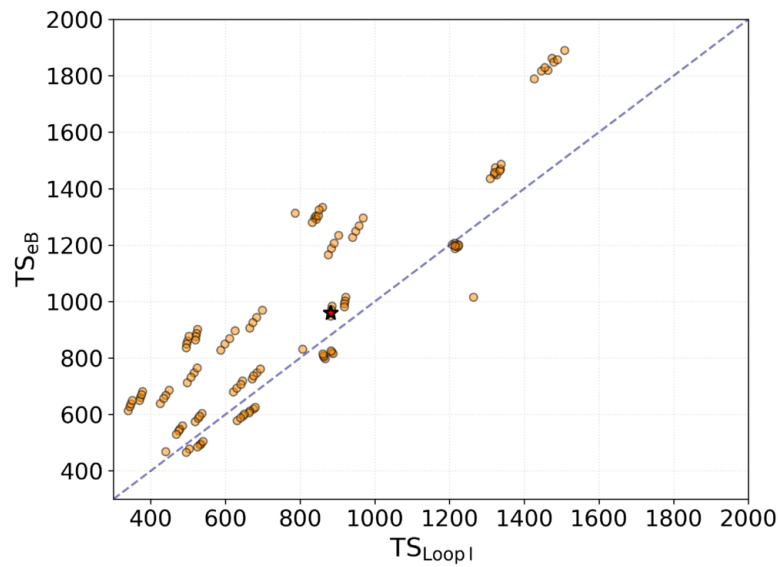
Figure A1. from Zhen Xie et al 2026 Astrophys. J. 1009 doi:10.3847/1538-4357/ae986d https://dx.doi.org/10.3847/1538-4357/ae986d © 2026. The Author(s). Published by the American Astronomical Society.
