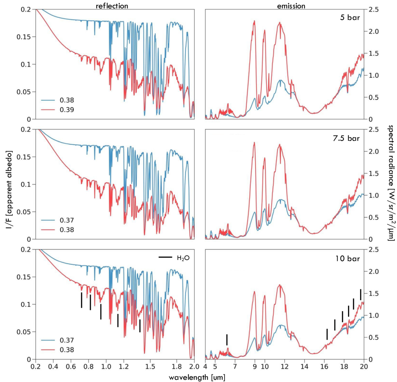
Figure 6. from Daria Pidhorodetska et al 2026 Astrophys. J. 1009 doi:10.3847/1538-4357/ae9869 https://dx.doi.org/10.3847/1538-4357/ae9869 © 2026. The Author(s). Published by the American Astronomical Society.
