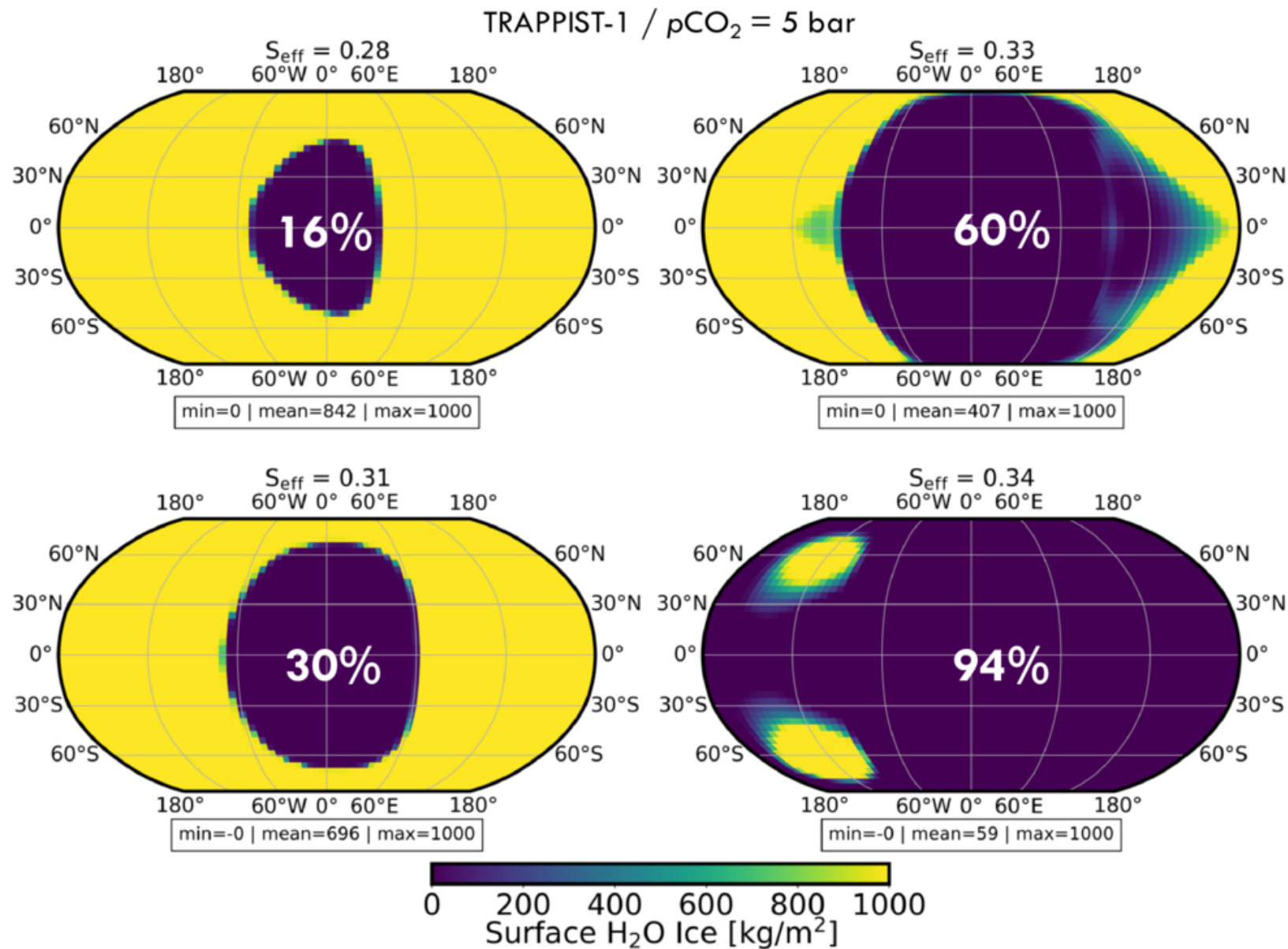
Figure 1. from Daria Pidhorodetska et al 2026 Astrophys. J. 1009 doi:10.3847/1538-4357/ae9869 https://dx.doi.org/10.3847/1538-4357/ae9869 © 2026. The Author(s). Published by the American Astronomical Society.
