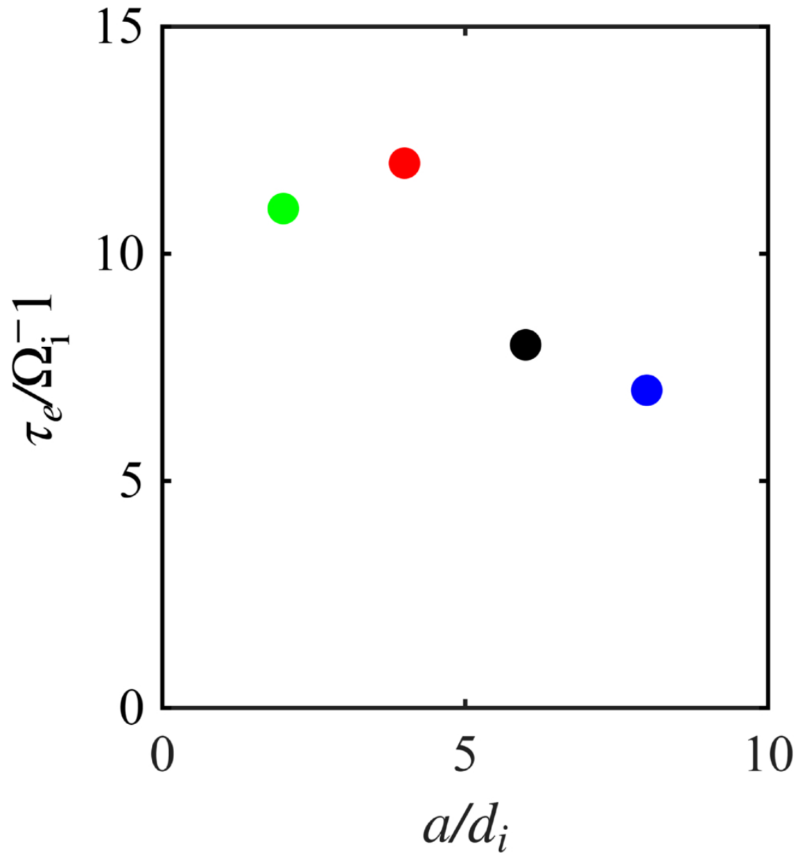
Figure 8. from Yundan Guan et al 2026 Astrophys. J. 1009 doi:10.3847/1538-4357/ae976b https://dx.doi.org/10.3847/1538-4357/ae976b © 2026. The Author(s). Published by the American Astronomical Society.
