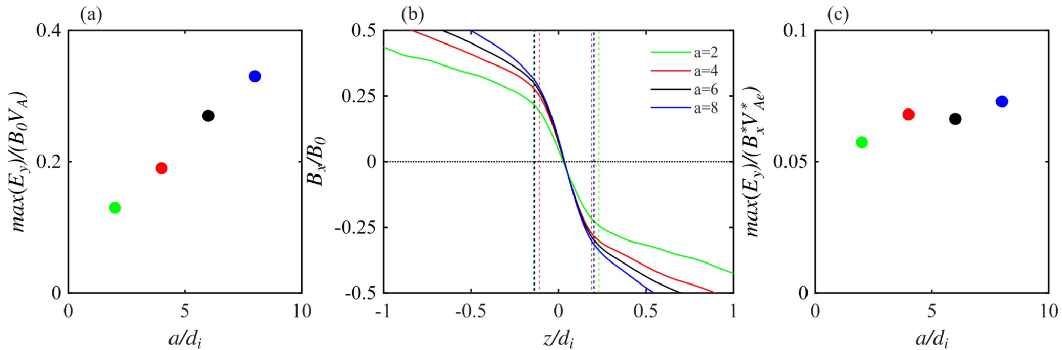
Figure 6. from Yundan Guan et al 2026 Astrophys. J. 1009 doi:10.3847/1538-4357/ae976b https://dx.doi.org/10.3847/1538-4357/ae976b © 2026. The Author(s). Published by the American Astronomical Society.
