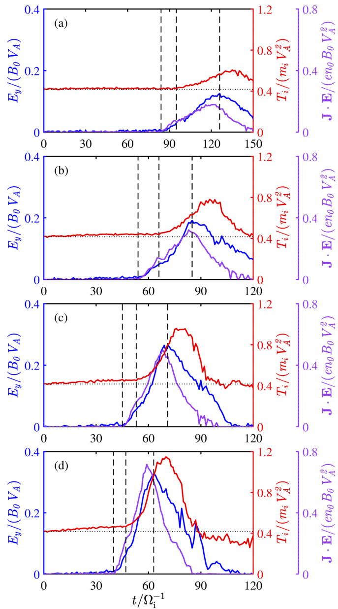
Figure 5. from Yundan Guan et al 2026 Astrophys. J. 1009 doi:10.3847/1538-4357/ae976b https://dx.doi.org/10.3847/1538-4357/ae976b © 2026. The Author(s). Published by the American Astronomical Society.
