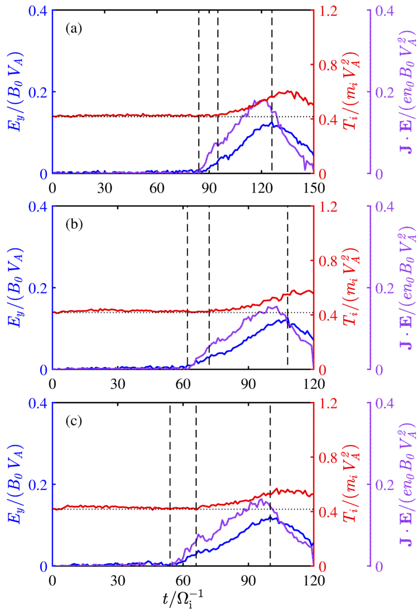
Figure 4. from Yundan Guan et al 2026 Astrophys. J. 1009 doi:10.3847/1538-4357/ae976b https://dx.doi.org/10.3847/1538-4357/ae976b © 2026. The Author(s). Published by the American Astronomical Society.
