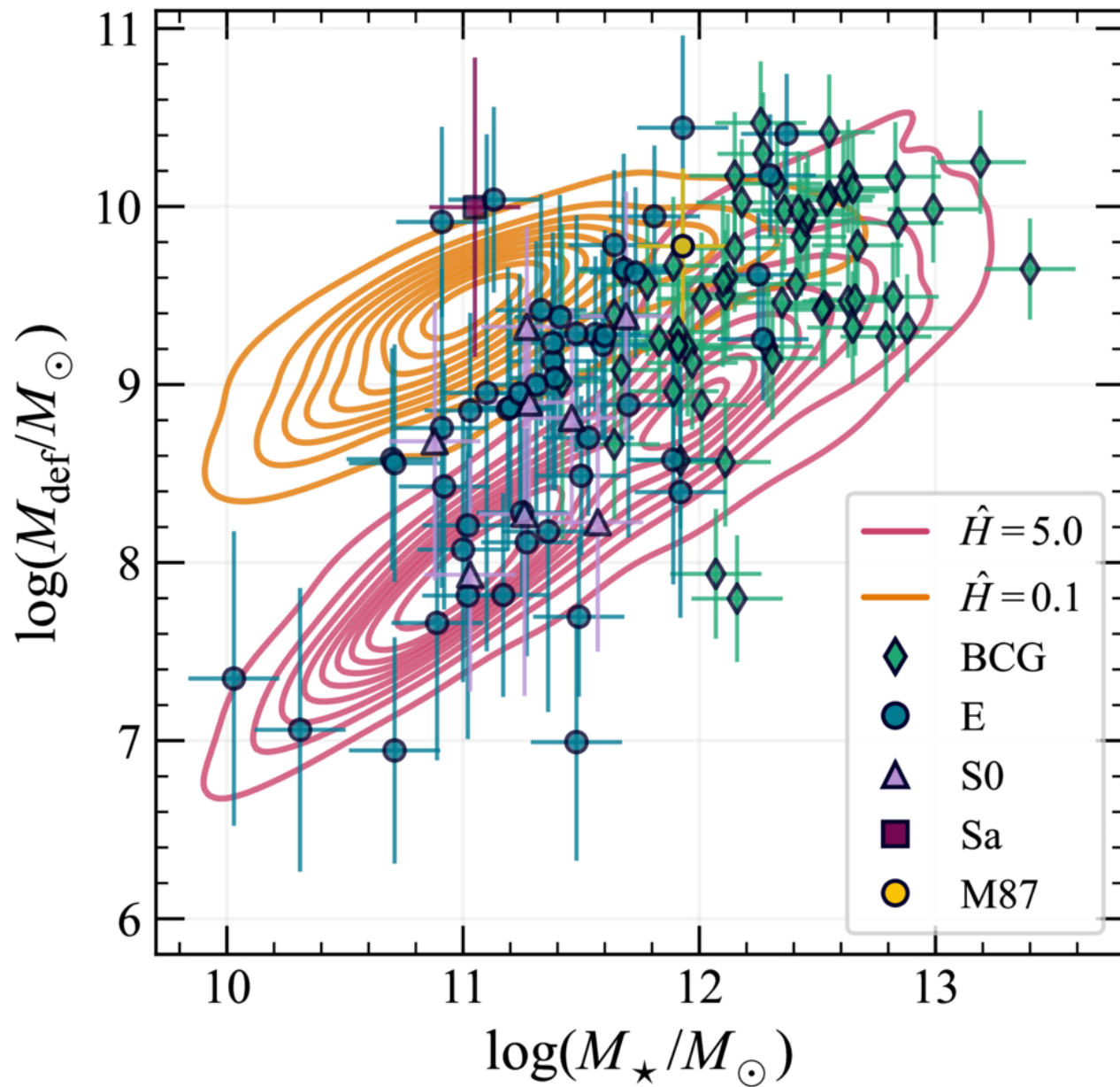
Figure 5. from C. J. Harris et al 2026 Astrophys. J. 1009 doi:10.3847/1538-4357/ae9767 https://dx.doi.org/10.3847/1538-4357/ae9767 © 2026. The Author(s). Published by the American Astronomical Society.
