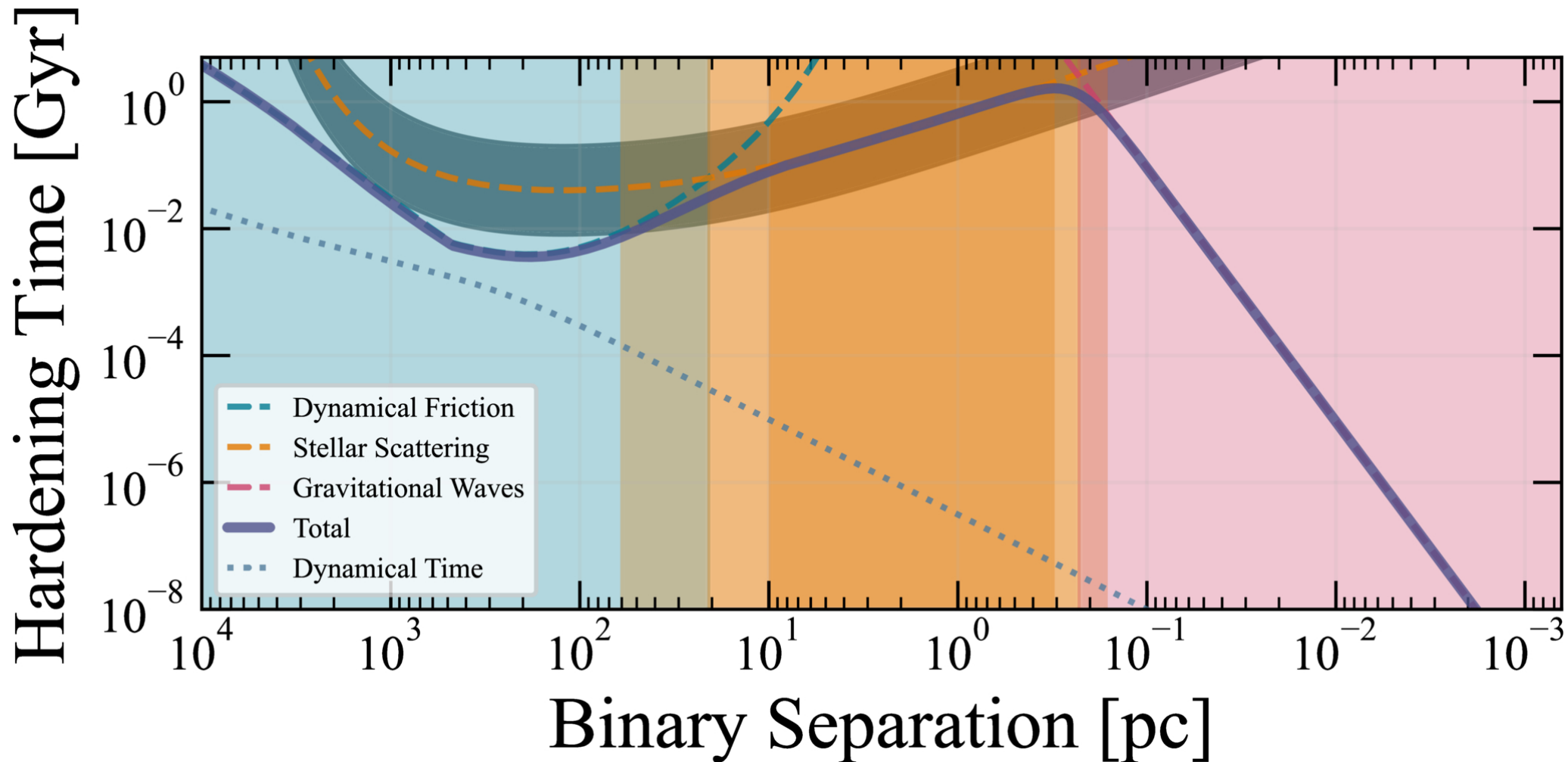
Figure 4. from C. J. Harris et al 2026 Astrophys. J. 1009 doi:10.3847/1538-4357/ae9767 https://dx.doi.org/10.3847/1538-4357/ae9767 © 2026. The Author(s). Published by the American Astronomical Society.
