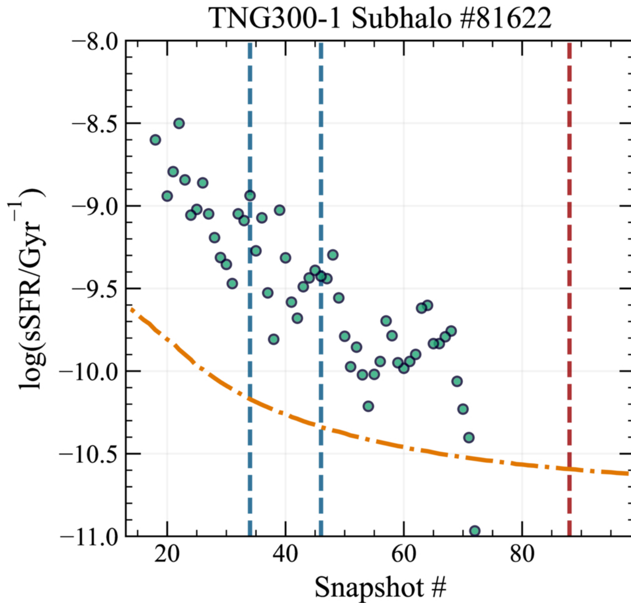
Figure 3. from C. J. Harris et al 2026 Astrophys. J. 1009 doi:10.3847/1538-4357/ae9767 https://dx.doi.org/10.3847/1538-4357/ae9767 © 2026. The Author(s). Published by the American Astronomical Society.
