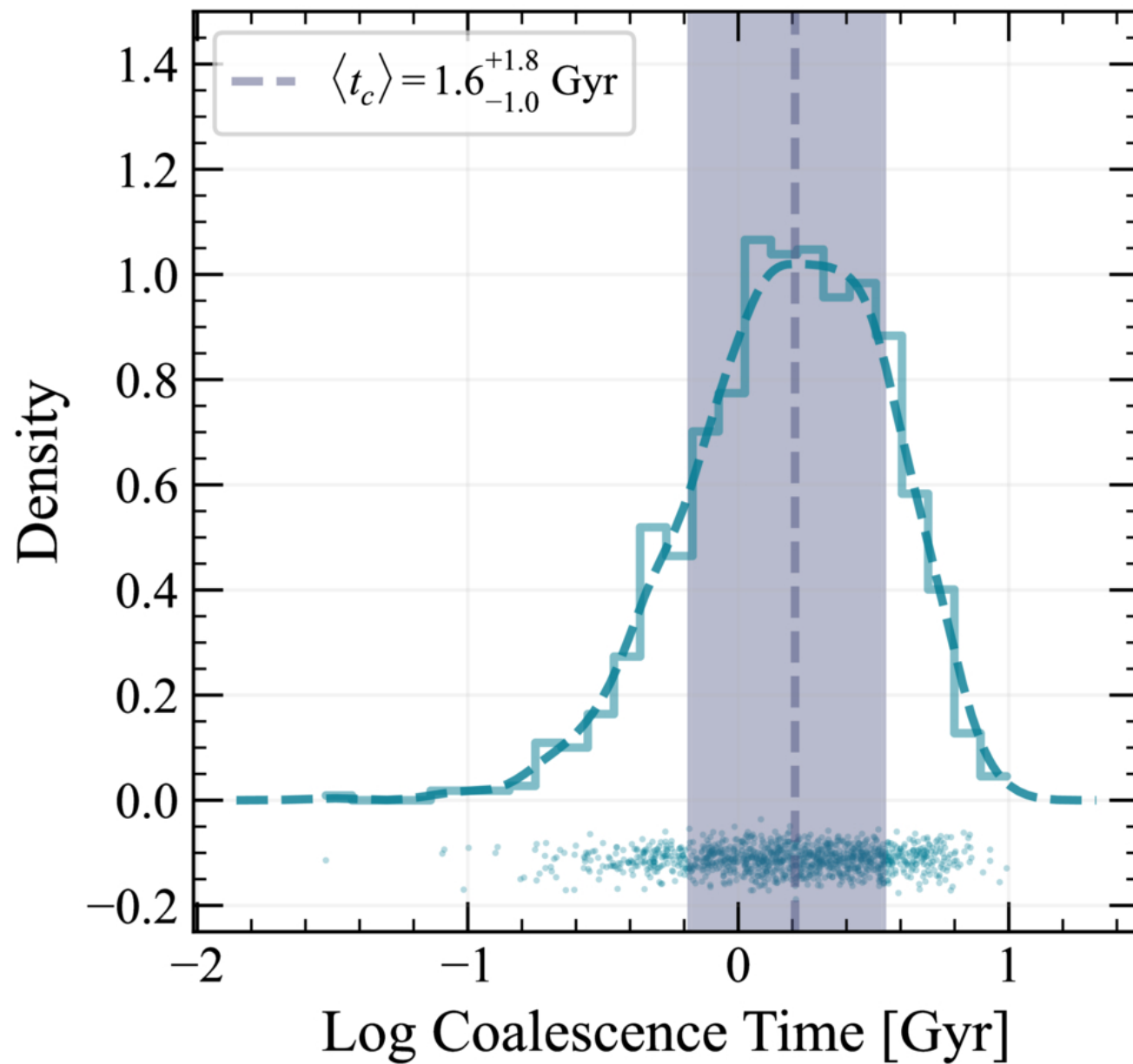
Figure 10. from C. J. Harris et al 2026 Astrophys. J. 1009 doi:10.3847/1538-4357/ae9767 https://dx.doi.org/10.3847/1538-4357/ae9767 © 2026. The Author(s). Published by the American Astronomical Society.
