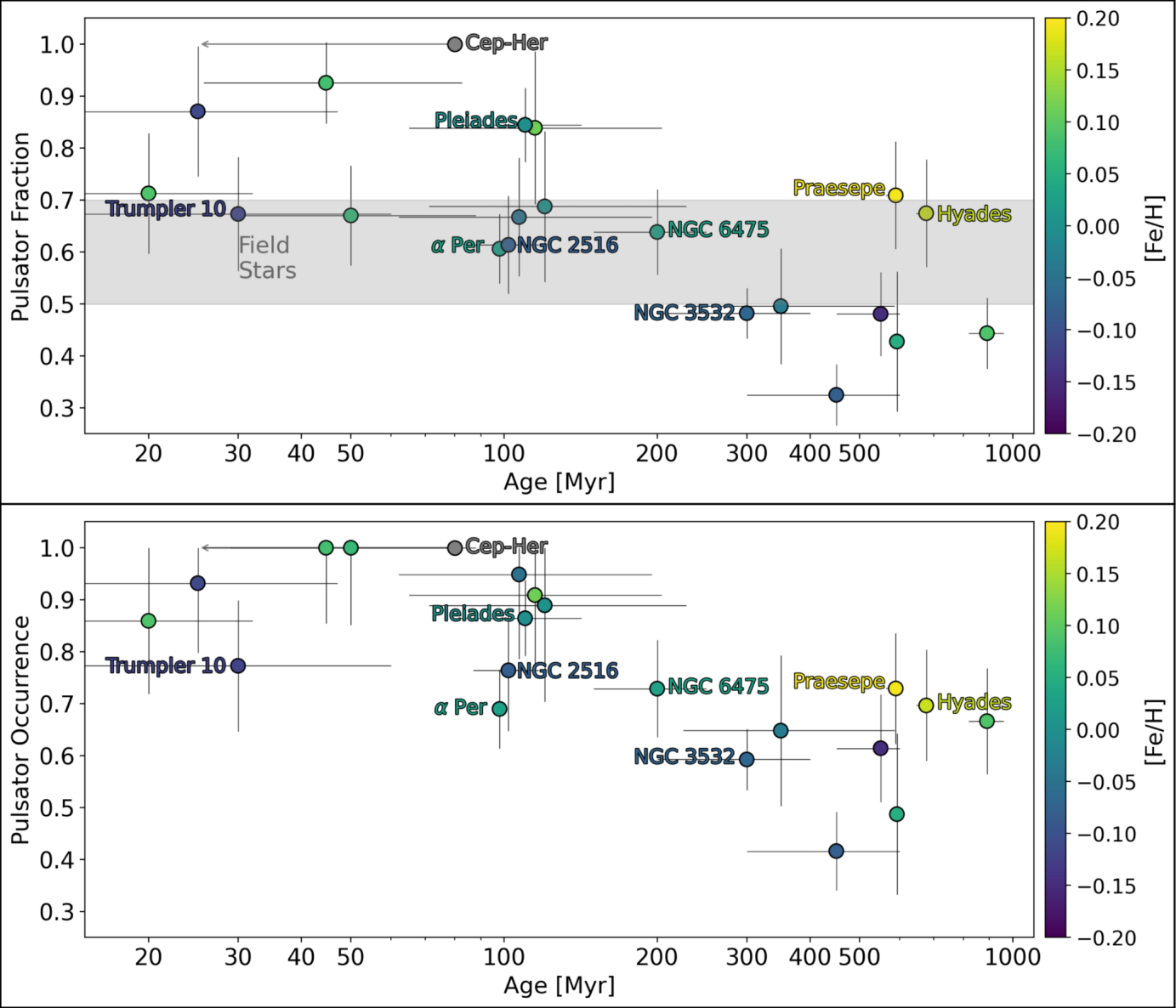
Figure 6. from Ian Berry et al 2026 Astrophys. J. 1009 doi:10.3847/1538-4357/ae9764 https://dx.doi.org/10.3847/1538-4357/ae9764 © 2026. The Author(s). Published by the American Astronomical Society.
