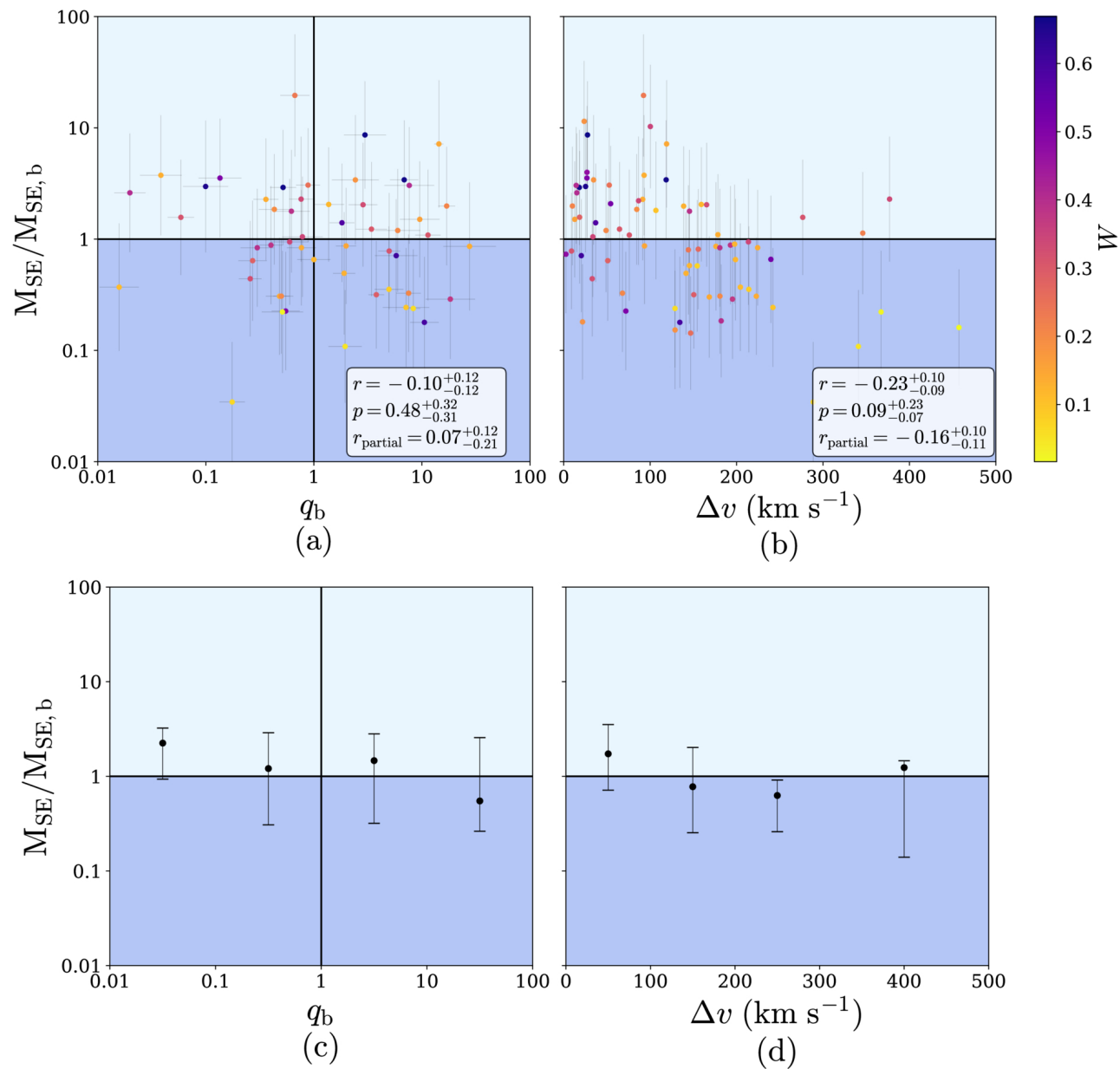
Figure 4. from Maggie C. Huber et al 2026 Astrophys. J. 1008 doi:10.3847/1538-4357/ae975b https://dx.doi.org/10.3847/1538-4357/ae975b © 2026. The Author(s). Published by the American Astronomical Society.
