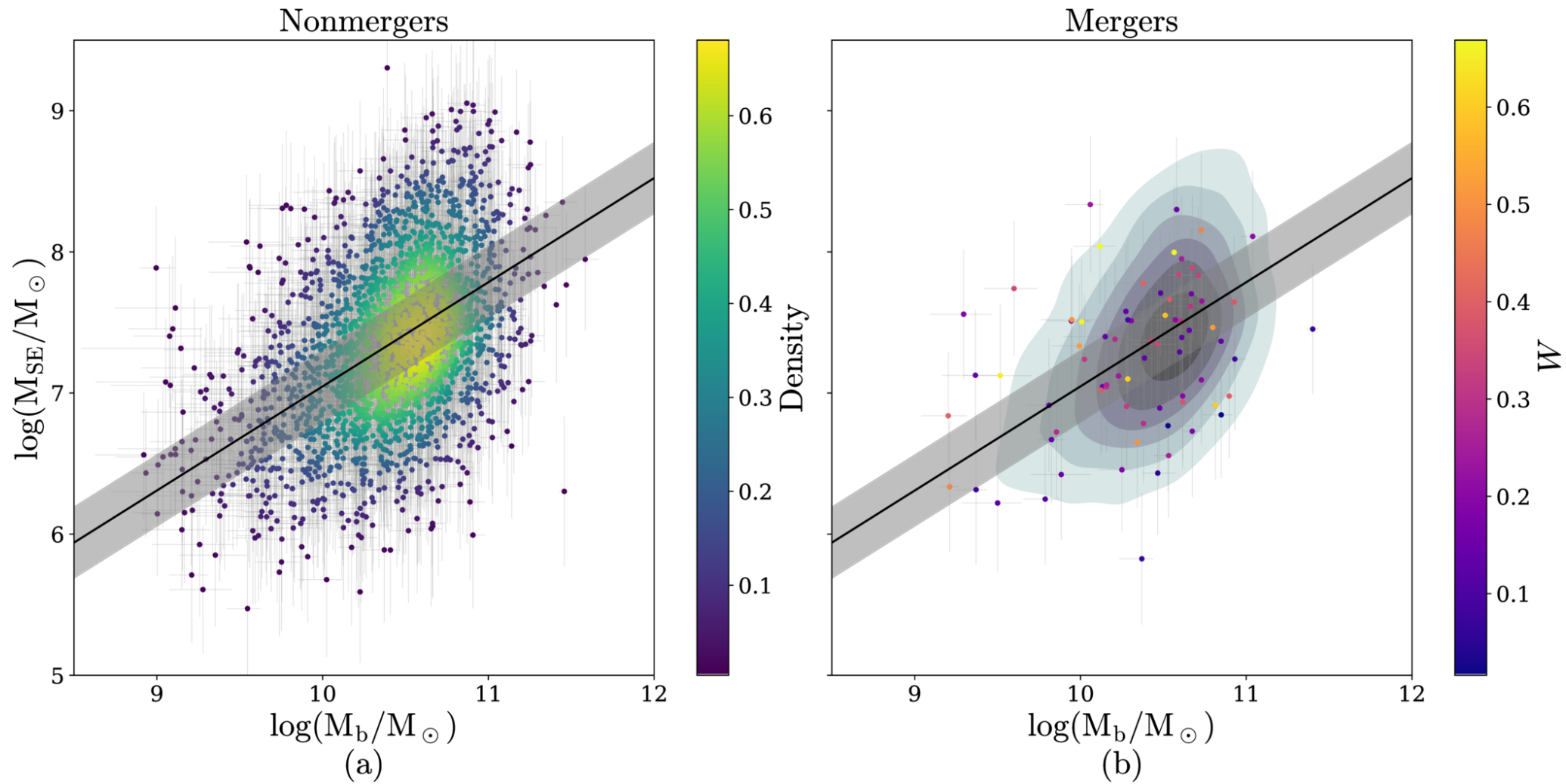
Figure 2. from Maggie C. Huber et al 2026 Astrophys. J. 1008 doi:10.3847/1538-4357/ae975b https://dx.doi.org/10.3847/1538-4357/ae975b © 2026. The Author(s). Published by the American Astronomical Society.
